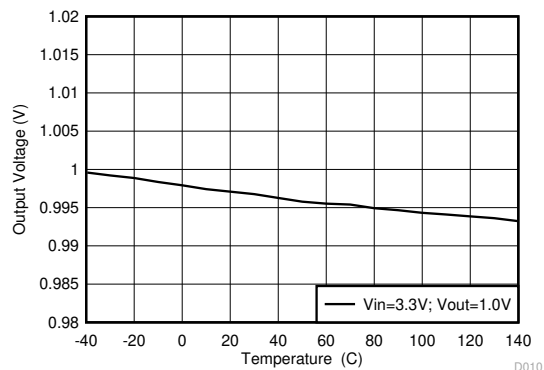
8-9. Buck Output Voltage vs Temperature
