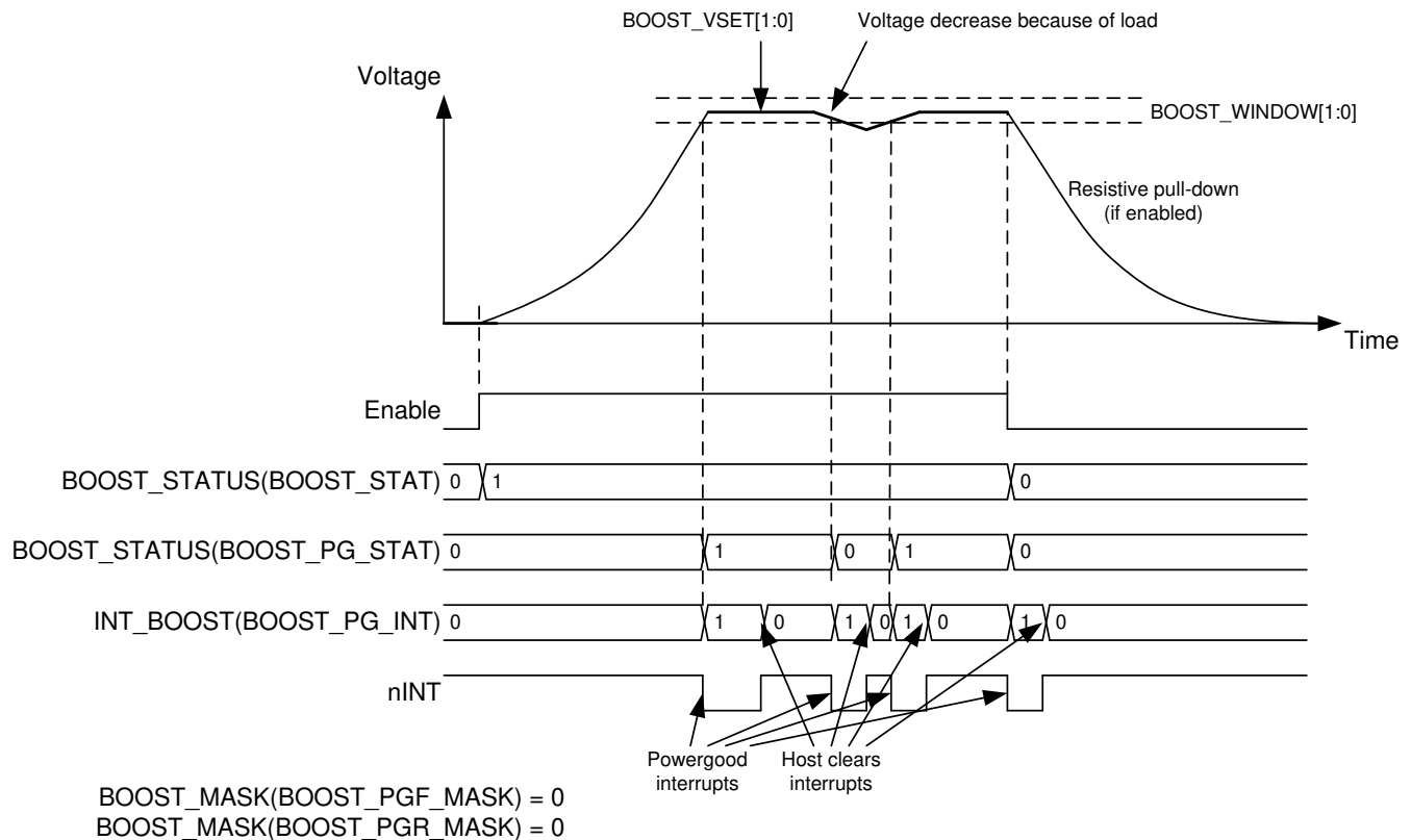
FIG 7-5. Boost Converter Enable and Disable
