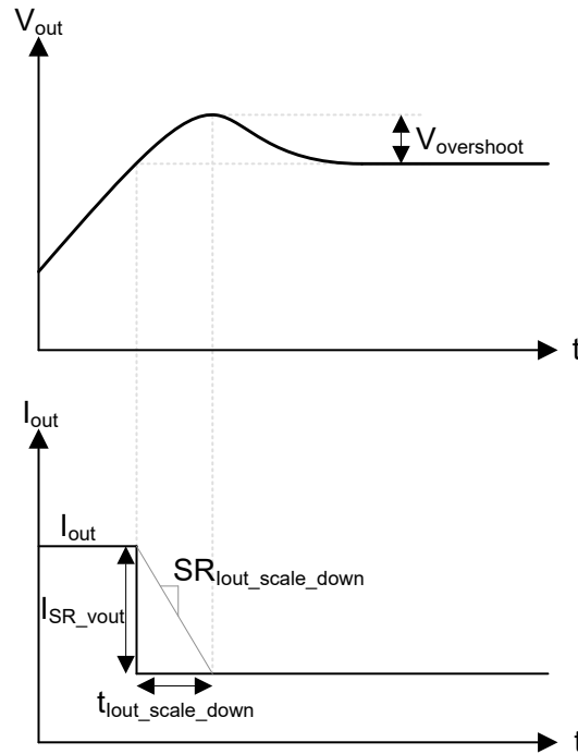
8-5. Overshoot
