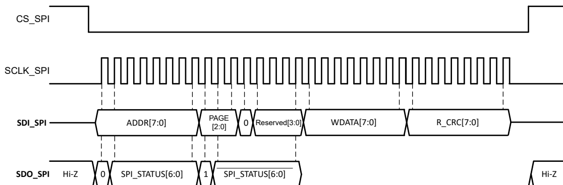
✎ 7-57. SPI Write Cycle with CRC
