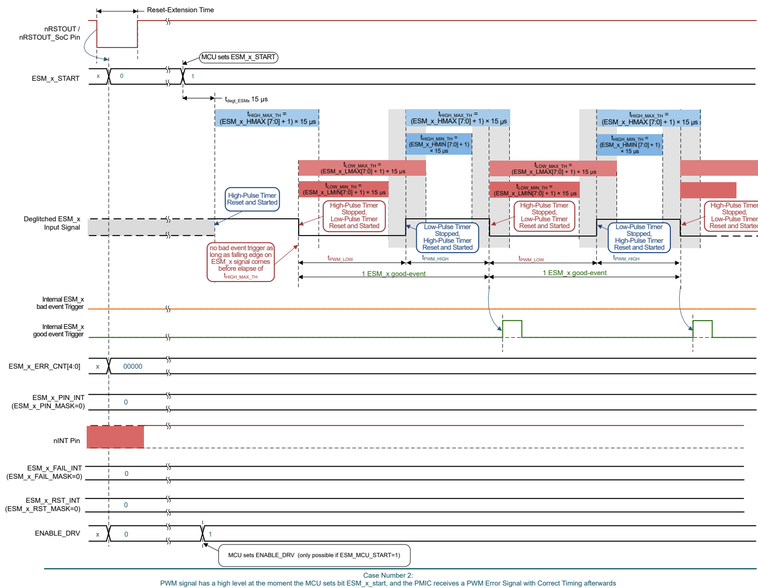
FIG 7-32. Example Waveform for ESM_MCU in PWM Mode – Case Number 2: ESM_MCU Starts with High-Level at Deglitched Input Signal, and Receives Correct PWM Signal Afterwards (The _x stand for _MCU)
