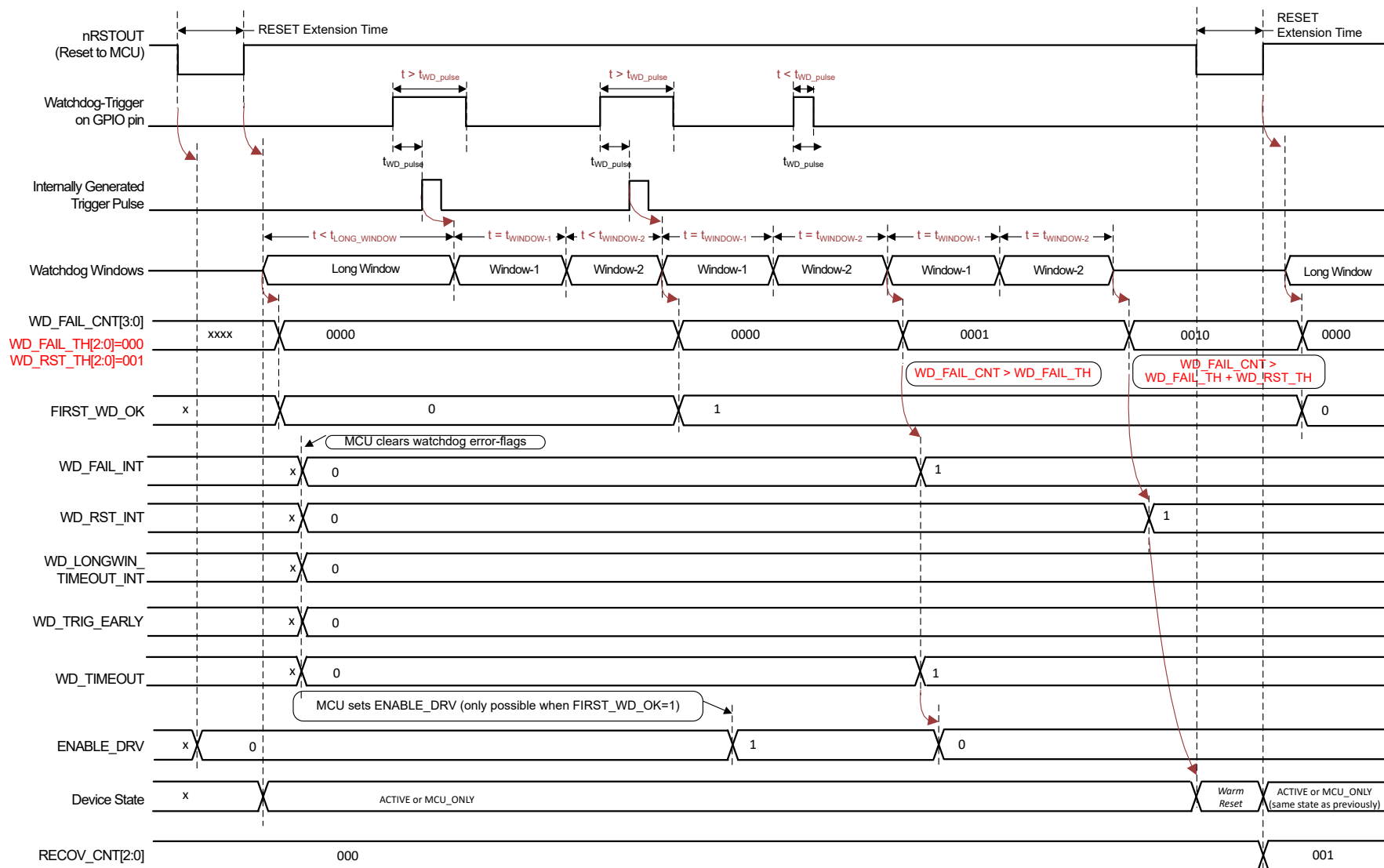
FIG 7-18. Watchdog in Trigger Mode – Bad Events (Too Short or no Trigger in Window-2) After Start-up
