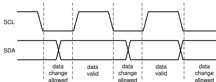
FIG 7-48. Data Validity Diagram
