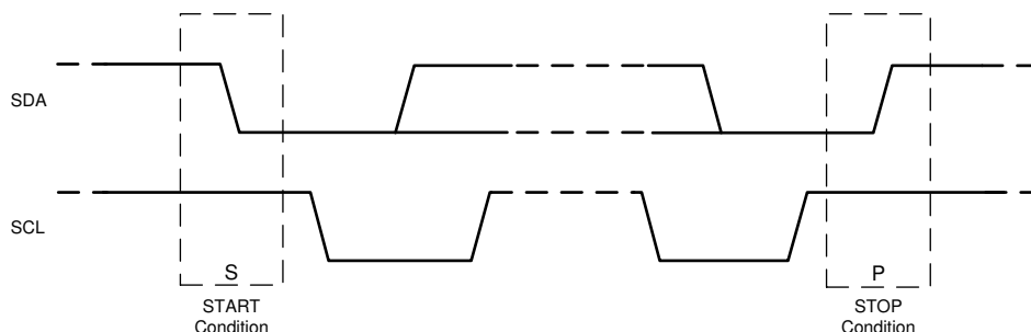
FIG 7-49. Start and Stop Sequences
