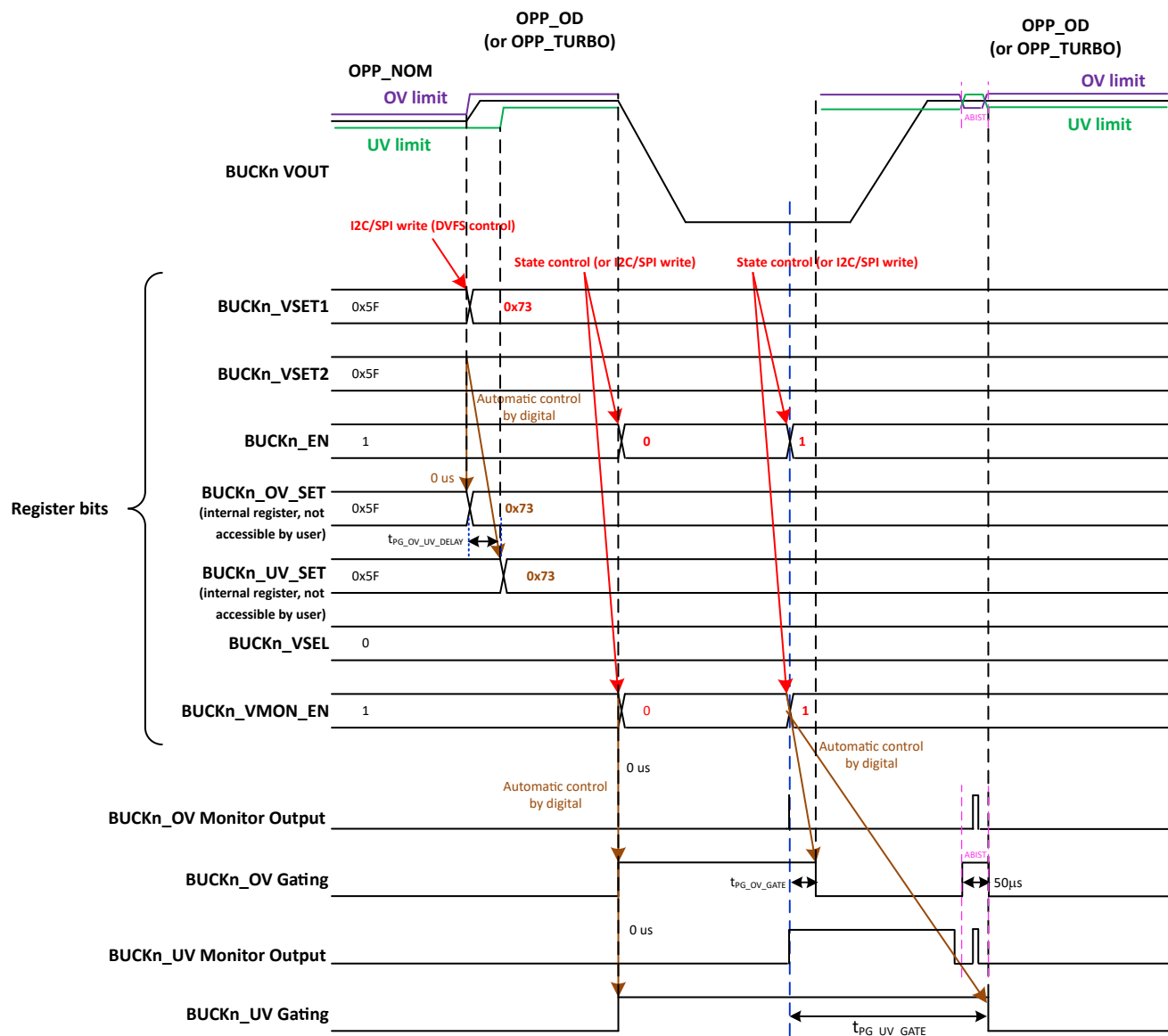
7-6. DVS Voltage and OV UV Threshold Level Change Timing Diagram
