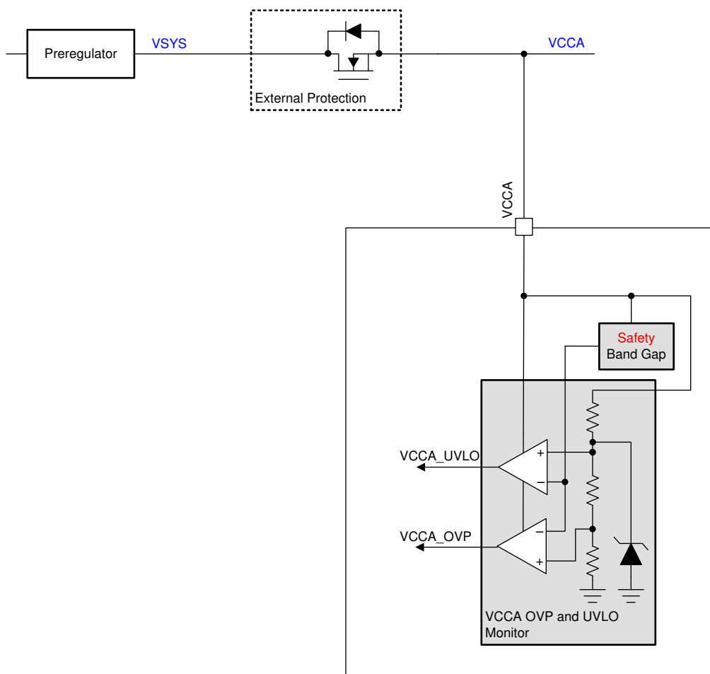
Figure 7-2. VCCA Monitor
