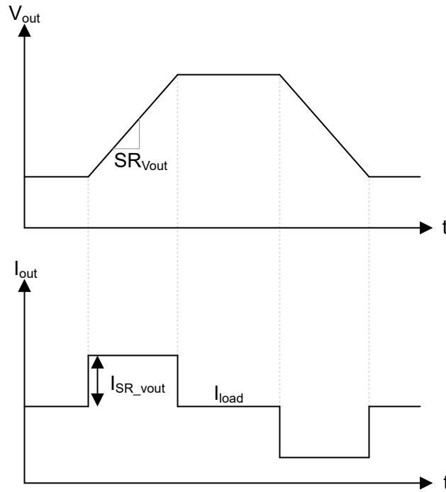
8-4. Voltage ramp
