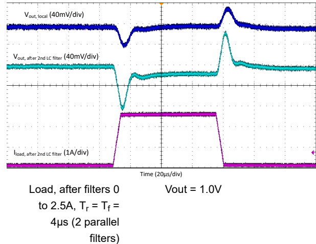
8-19. Load Transient Response, FPWM Mode. 8.8 MHz Single Phase.
