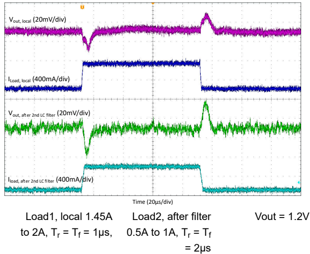
8-18. Load Transient Response, FPWM Mode. 8.8 MHz Single Phase.
