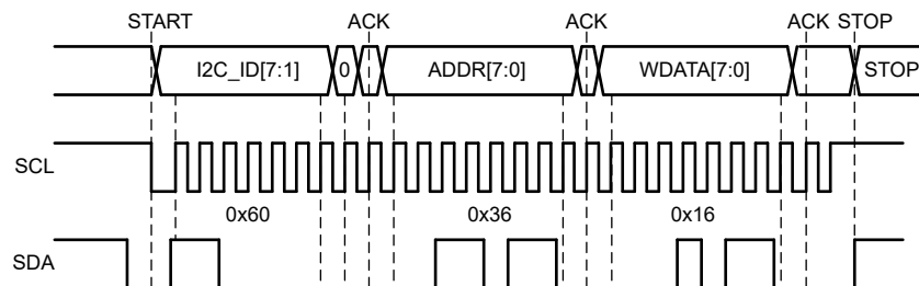
FIG 7-52. I 2 C Write Cycle without CRC
