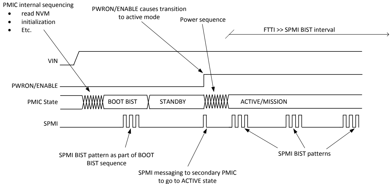
7-45. SPMI-BIST Operation
