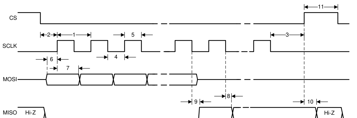
6-2. SPI Timing
