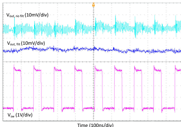
8-13. Output Voltage Ripple 8.8 MHz Single Phase. FPWM mode. L = 100 nH.
