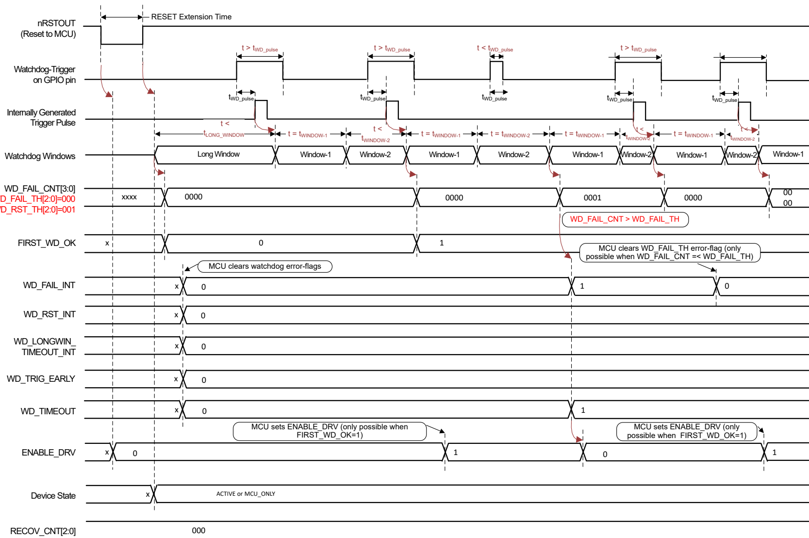
FIG 7-19. Watchdog in Trigger Mode – Good Events (Correct Watchdog-Triggers) After Start-up, Followed by a Bad-Event (No Watchdog-Trigger in Window-2) and After That Followed by a Good Event.
