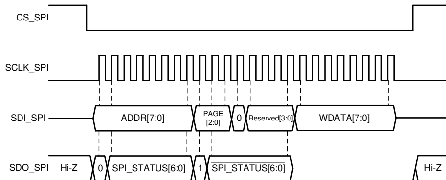
✎ 7-56. SPI Write Cycle
