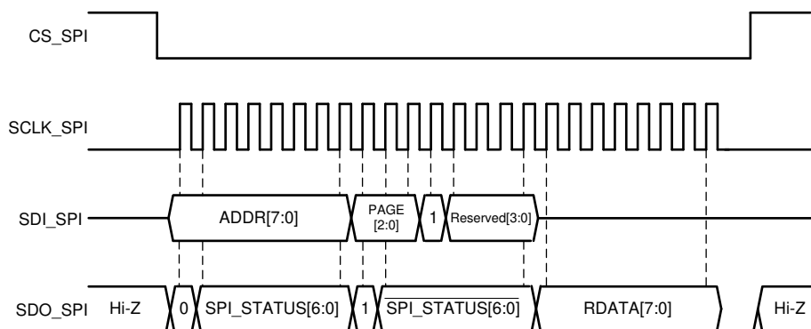
✎ 7-58. SPI Read Cycle
