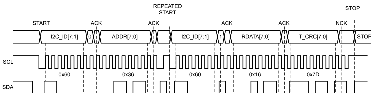
FIG 7-54. I 2 C Read Cycle without CRC
