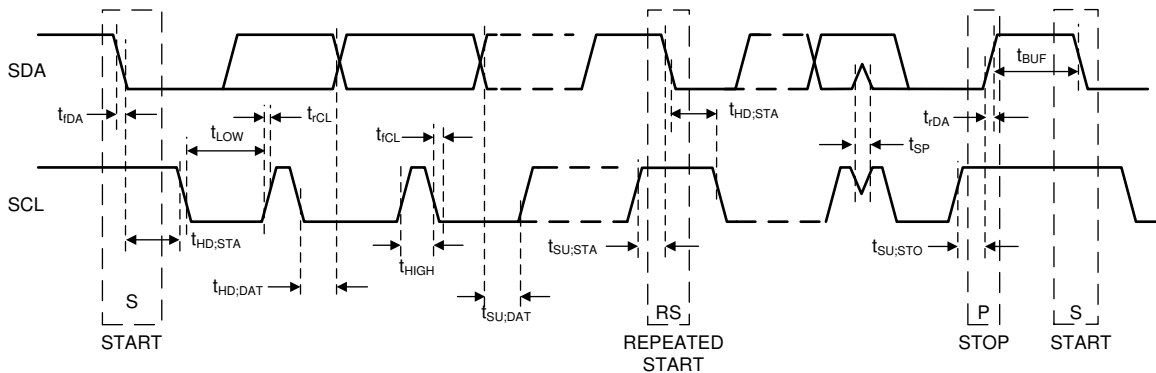
FIG 6-1. I 2 C Timing
