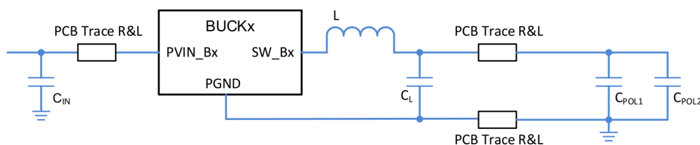
図 8-2. Buck Regulators Power Distribution Network (PDN)
