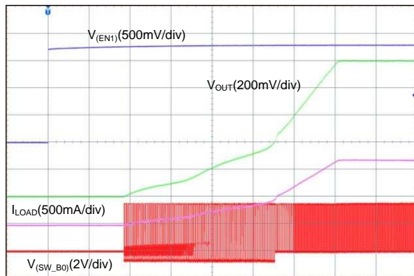
☒ 70. Start-Up With EN1, Forced PWM (3-Phase Output)
