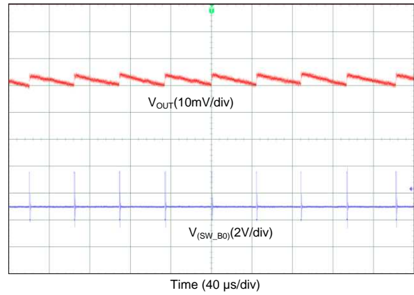
Figure 77. Output Voltage Ripple, PFM Mode (4-Phase Output)
