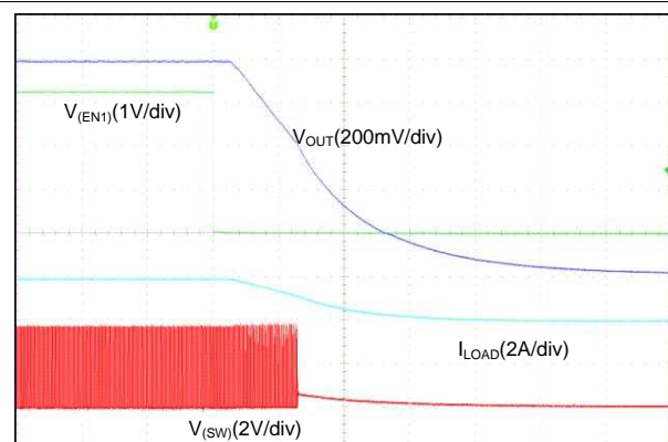
☒ 73. Shutdown With EN1, Forced PWM (4-Phase Output)
