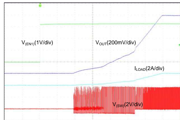
☒ 71. Start-Up With EN1, Forced PWM (2-Phase Output)
