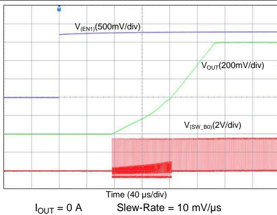
图 68. Start-Up With EN1, Forced PWM (1-Phase Output)
