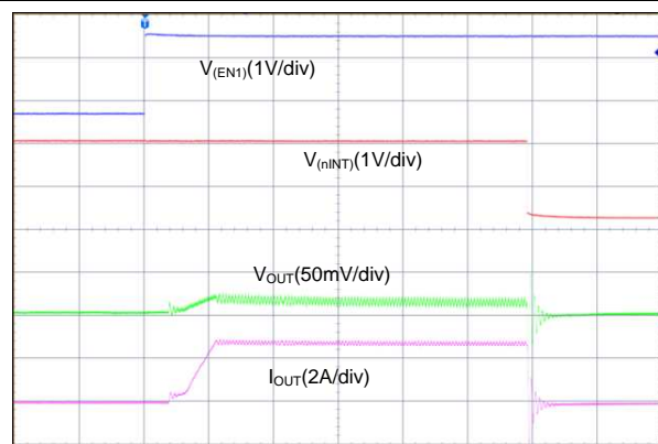
Time (200 \mu\text{s}/\text{div} )
