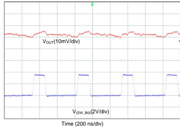
⊗ 83. Output Voltage Ripple, Forced-PWM Mode (2-Phase Output)
