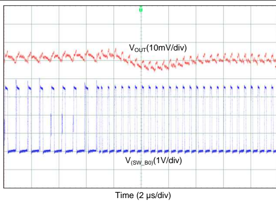
⊗ 86. Transient from PFM-to-PWM Mode (3-Phase Output)
