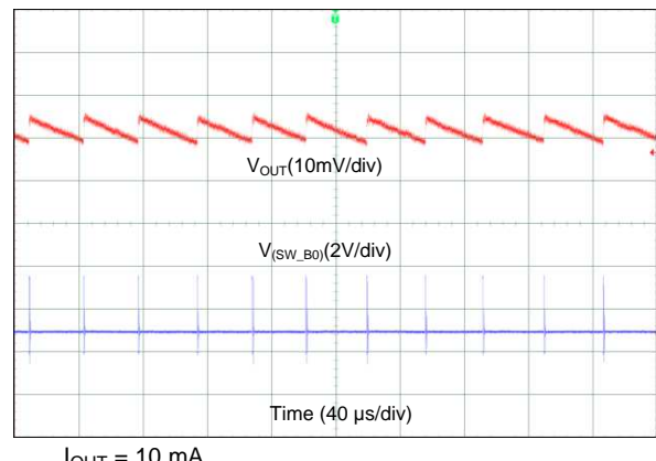
Figure 79. Output Voltage Ripple, PFM Mode (2-Phase Output)
