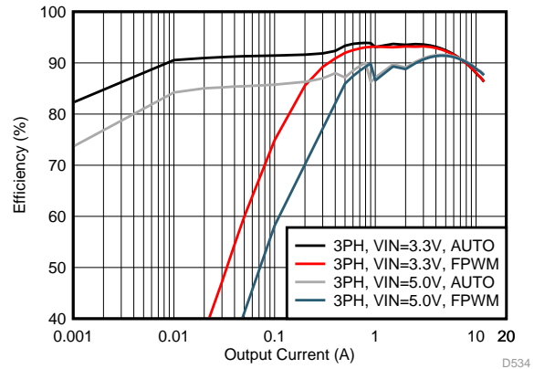
35. Efficiency in PFM/PWM and Forced-PWM Mode (3-Phase Output)
