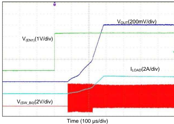
☒ 70. Start-Up With EN1, Forced PWM (3-Phase Output)
