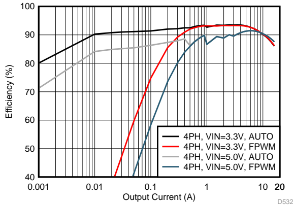
34. Efficiency in PFM/PWM and Forced-PWM Mode (4-Phase Output)
