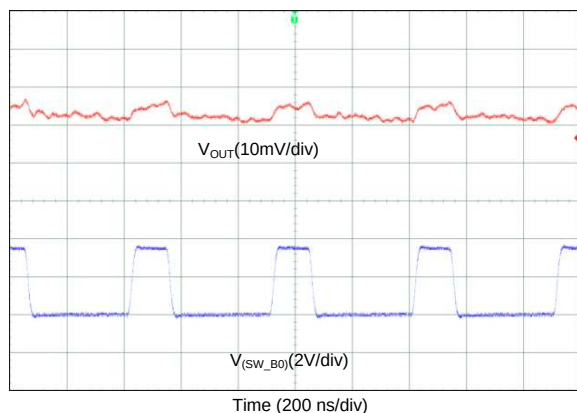
FIG 82. Output Voltage Ripple, Forced-PWM Mode (3-Phase Output)
