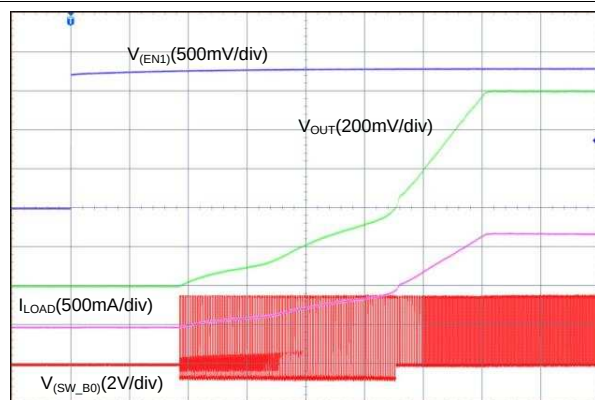
FIG 70. Start-Up With EN1, Forced PWM (3-Phase Output)
