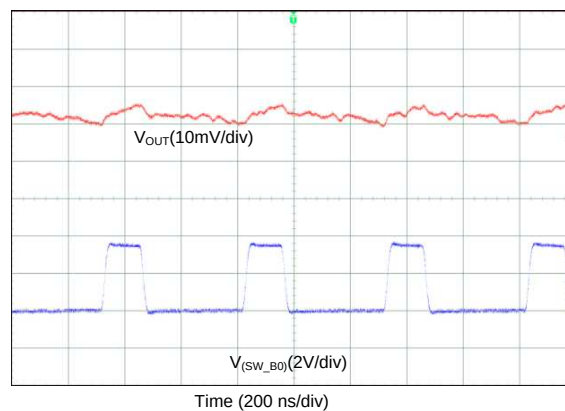
FIG 83. Output Voltage Ripple, Forced-PWM Mode (2-Phase Output)
