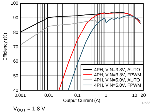
FIG 34. Efficiency in PFM/PWM and Forced-PWM Mode (4-Phase Output)
