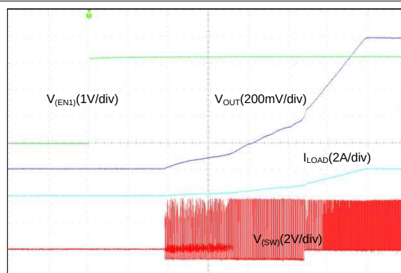
FIG 71. Start-Up With EN1, Forced PWM (2-Phase Output)
