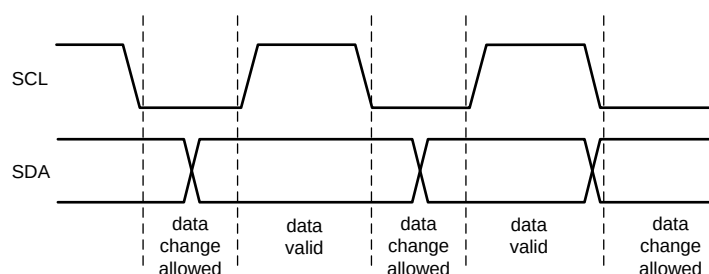
FIG 22. Data Validity Diagram
