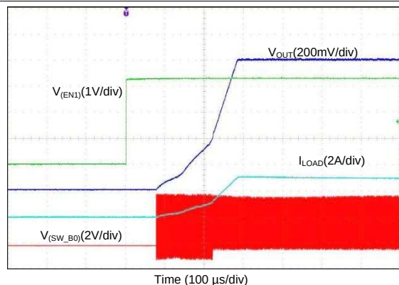
FIG 70. Start-Up With EN1, Forced PWM (3-Phase Output)
