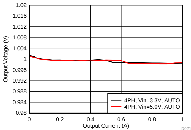
FIG 50. Output Voltage vs Load Current in PFM/PWM Mode (4-Phase Output)
