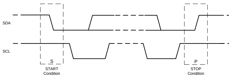
FIG 23. Start and Stop Sequences
