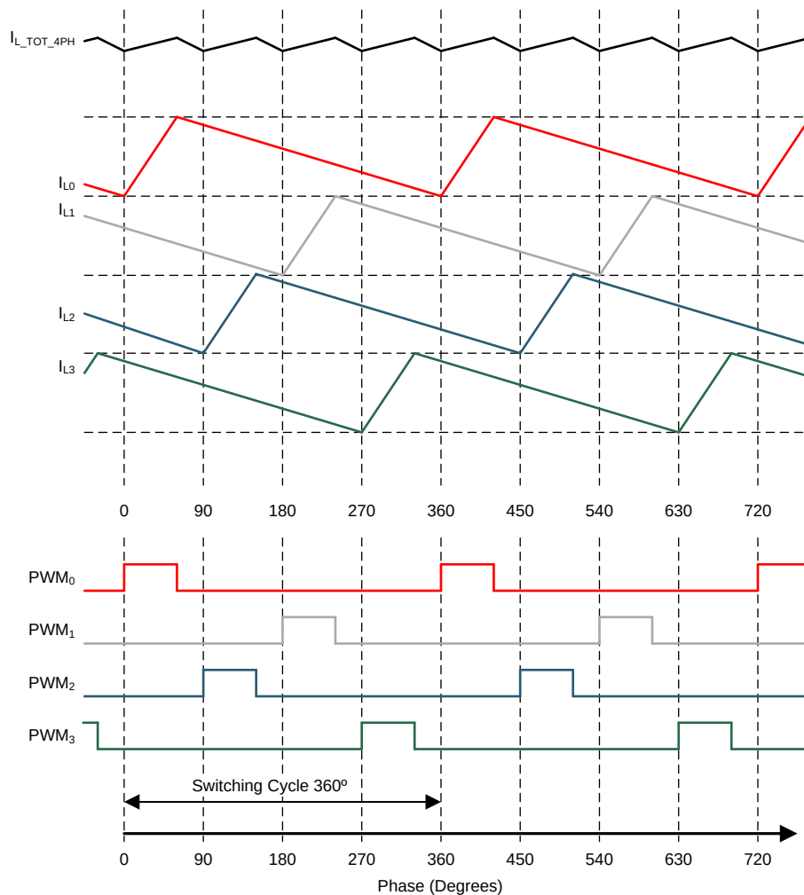
FIG 10. Example of PWM Timings, Inductor Current Waveforms, and Total Output Current in 4-Phase Configuration.
