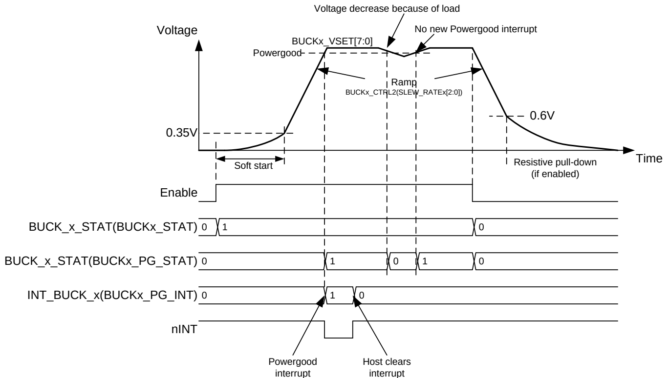
FIG 14. Regulator Enable and Disable
