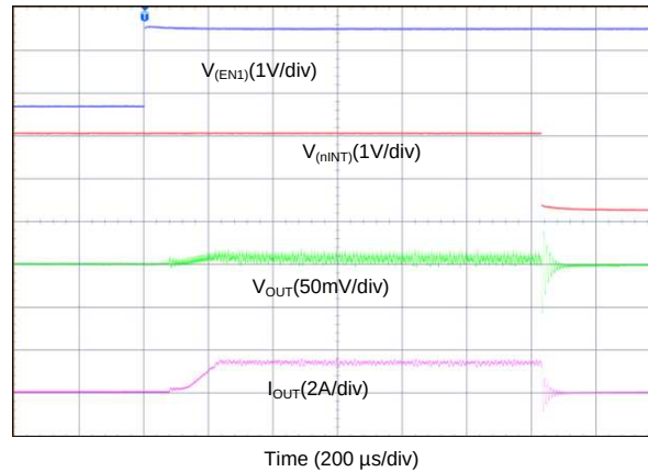
✎ 112. Start-Up With Short on Output (1-Phase Output)
