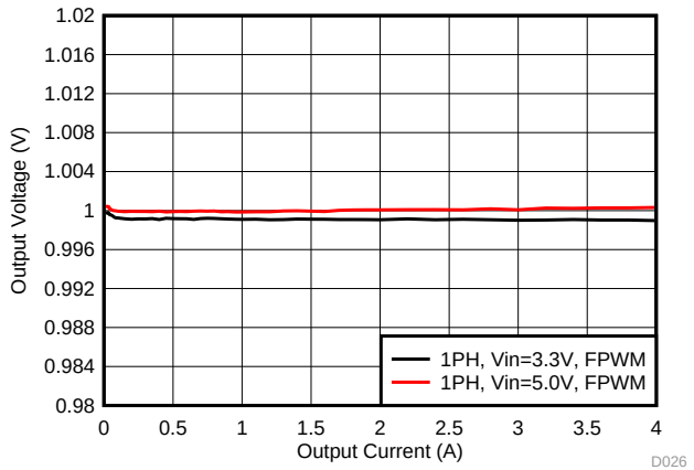
FIG 49. Output Voltage vs Load Current in Forced-PWM Mode (1-Phase Output)
