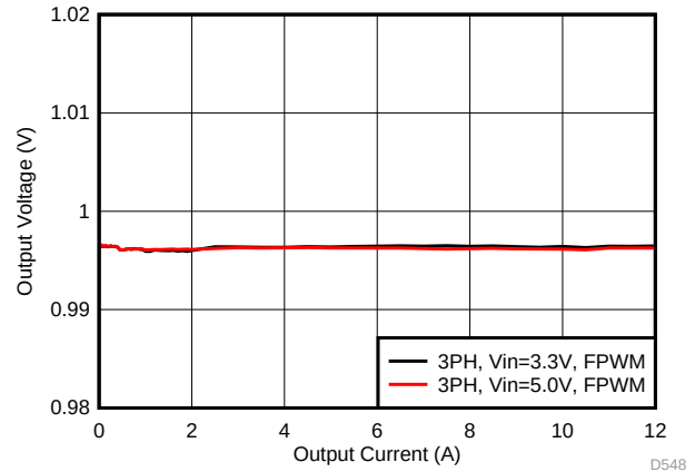
FIG 47. Output Voltage vs Load Current in Forced-PWM Mode (3-Phase Output)
