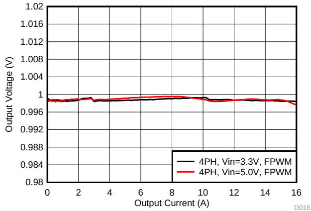
FIG 46. Output Voltage vs Load Current in Forced-PWM Mode (4-Phase Output)
