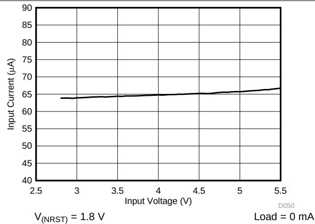
FIG 8. PFM Mode Current Consumption vs Input Voltage, One Regulator Enabled (2+2-Phase Output)
