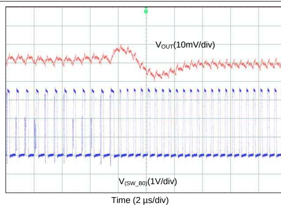
FIG 87. Transient from PFM-to-PWM Mode (2-Phase Output)
