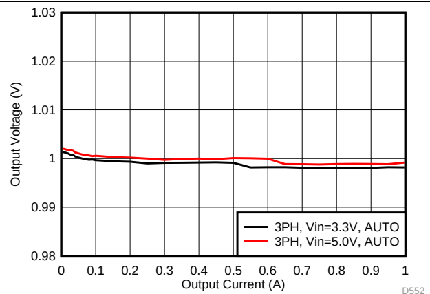
FIG 51. Output Voltage vs Load Current in PFM/PWM Mode (3-Phase Output)
