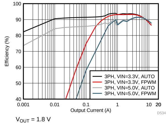
FIG 35. Efficiency in PFM/PWM and Forced-PWM Mode (3-Phase Output)
