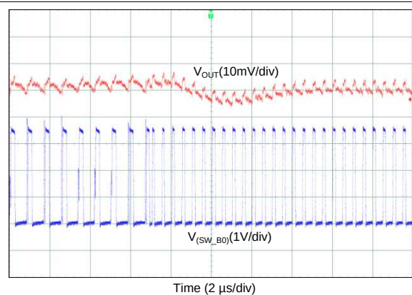
FIG 84. Output Voltage Ripple, Forced-PWM Mode (1-Phase Output)
