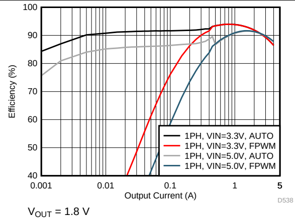
FIG 37. Efficiency in PFM/PWM and Forced-PWM Mode (1-Phase Output)
