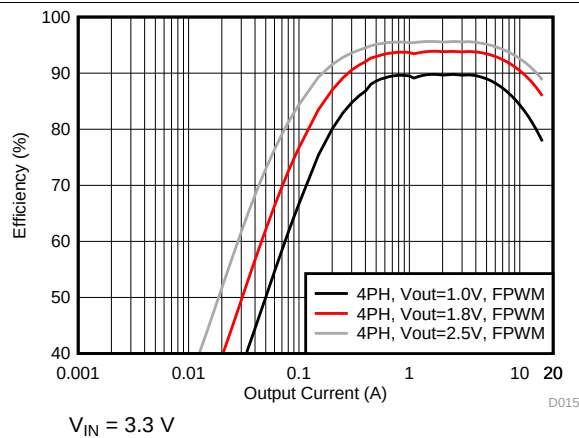
FIG 38. Efficiency in Forced-PWM Mode (4-Phase Output)
