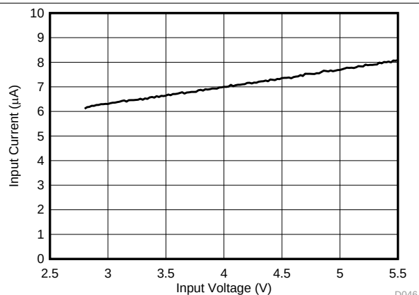
图 3. Standby Current Consumption vs Input Voltage
