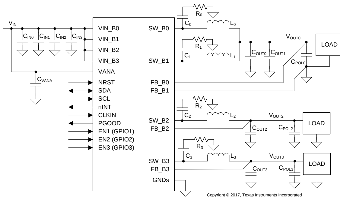
FIG 30. 2-Phase and Two 1-Phase Configuration (LP87563-Q1)
