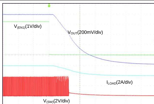
FIG 73. Shutdown With EN1, Forced PWM (4-Phase Output)
