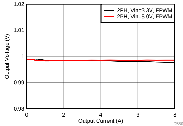
FIG 48. Output Voltage vs Load Current in Forced-PWM Mode (2-Phase Output)
