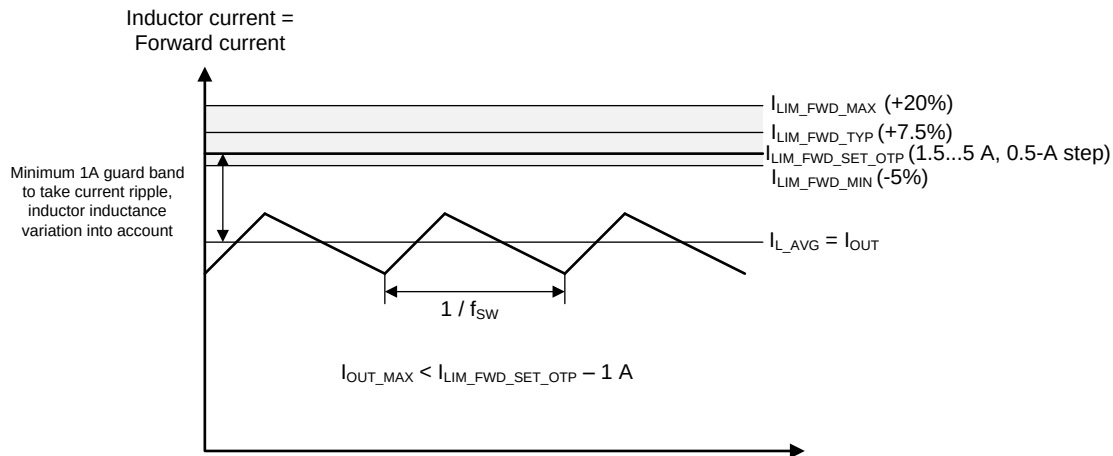
図 33. Current Limit vs Maximum Output Current
