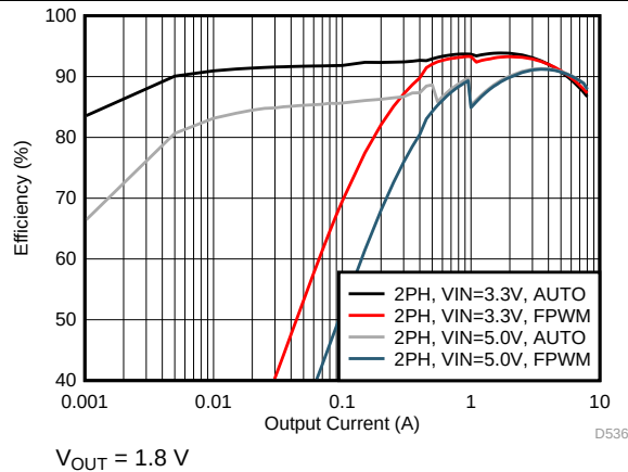
FIG 36. Efficiency in PFM/PWM and Forced-PWM Mode (2-Phase Output)
