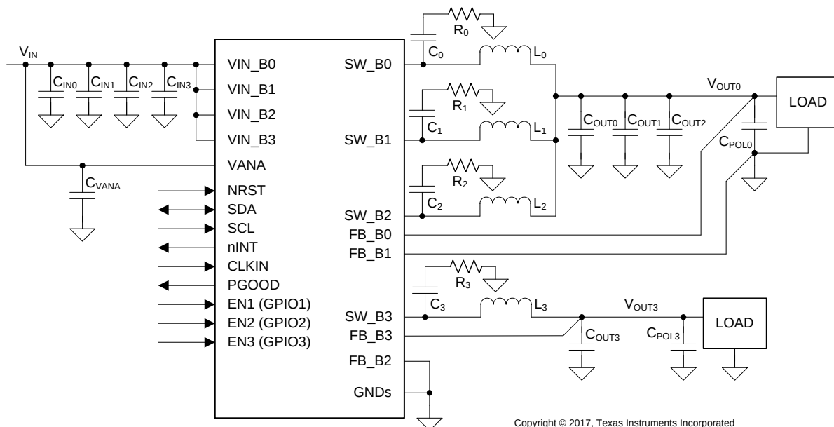
FIG 29. 3-Phase and 1-Phase Configuration (LP87562-Q1)
