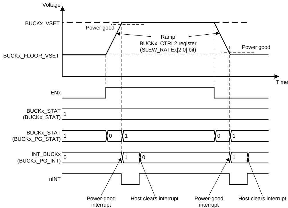
15. Regulator Output Voltage Change With ENx pin
