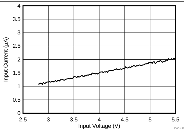
图 2. Shutdown Current Consumption vs Input Voltage
