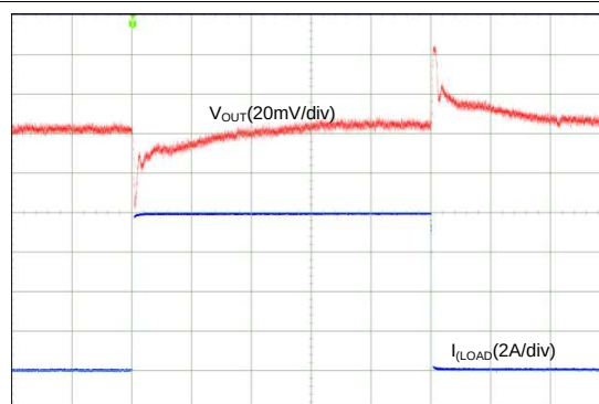
✎ 101. Transient Load Step Response, AUTO Mode (2-Phase Output)
