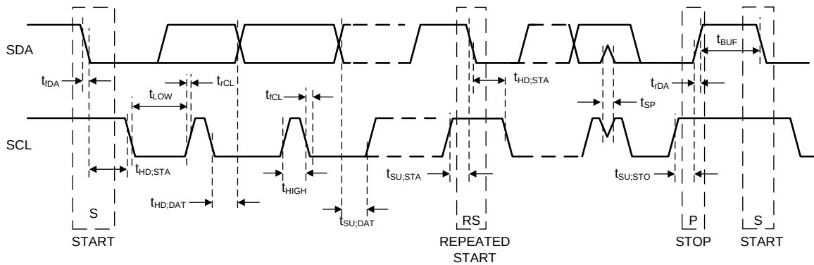
FIG 1. I 2 C Timing
