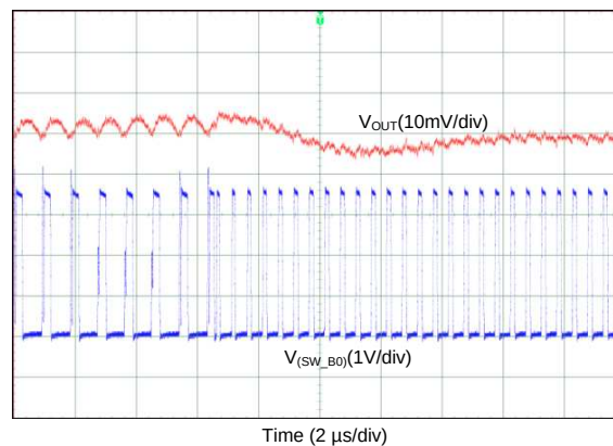
FIG 85. Transient from PFM-to-PWM Mode (4-Phase Output)
