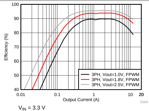
FIG 39. Efficiency in Forced-PWM Mode (3-Phase Output)
