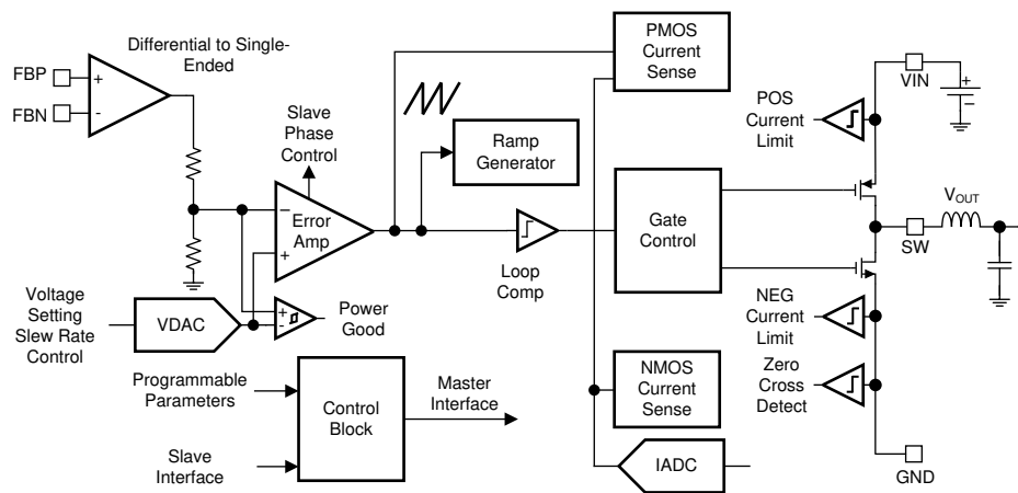
Figure 5. Detailed Block Diagram Showing One Core
