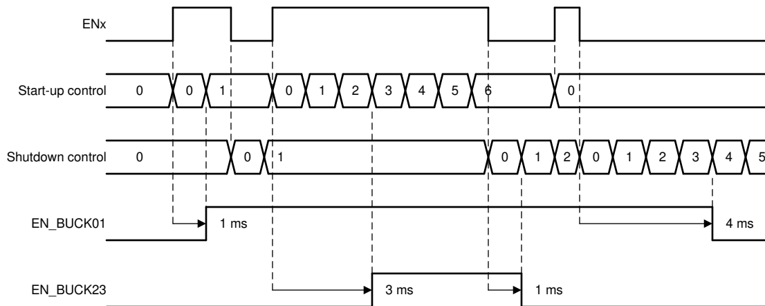
図 11. Start-Up and Shutdown Sequencing With Short ENx Low and High Periods
