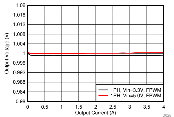
Figure 26. Output Voltage vs Load Current in Forced-PWM Mode
