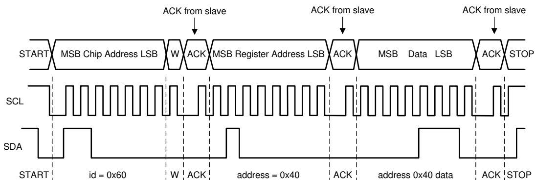
✎ 19. Write Cycle (w = write; SDA = 0), id = Device Address = 0x60 for LP87524B/J/P-Q1
