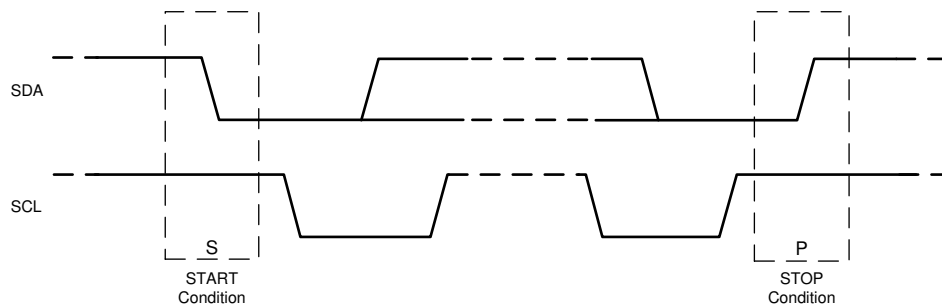
FIG 17. Start and Stop Sequences
