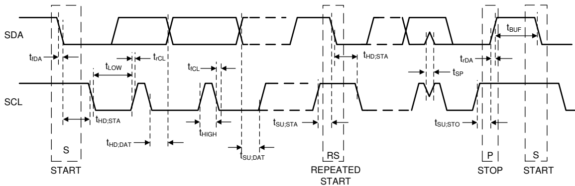
✎ 18. I²C-Compatible Timing
