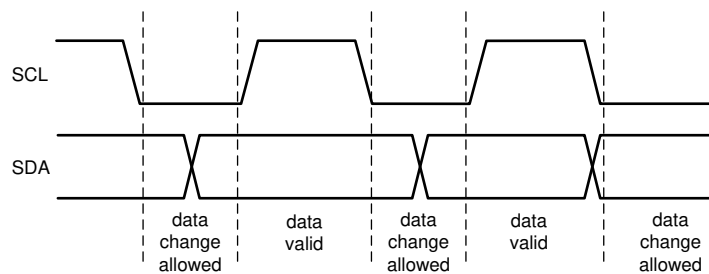
FIG 16. Data Validity Diagram
