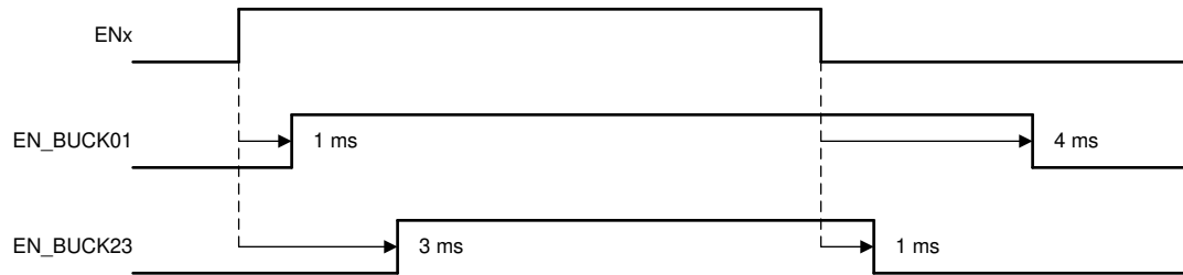
図 10. Typical Start-Up and Shutdown Sequencing
