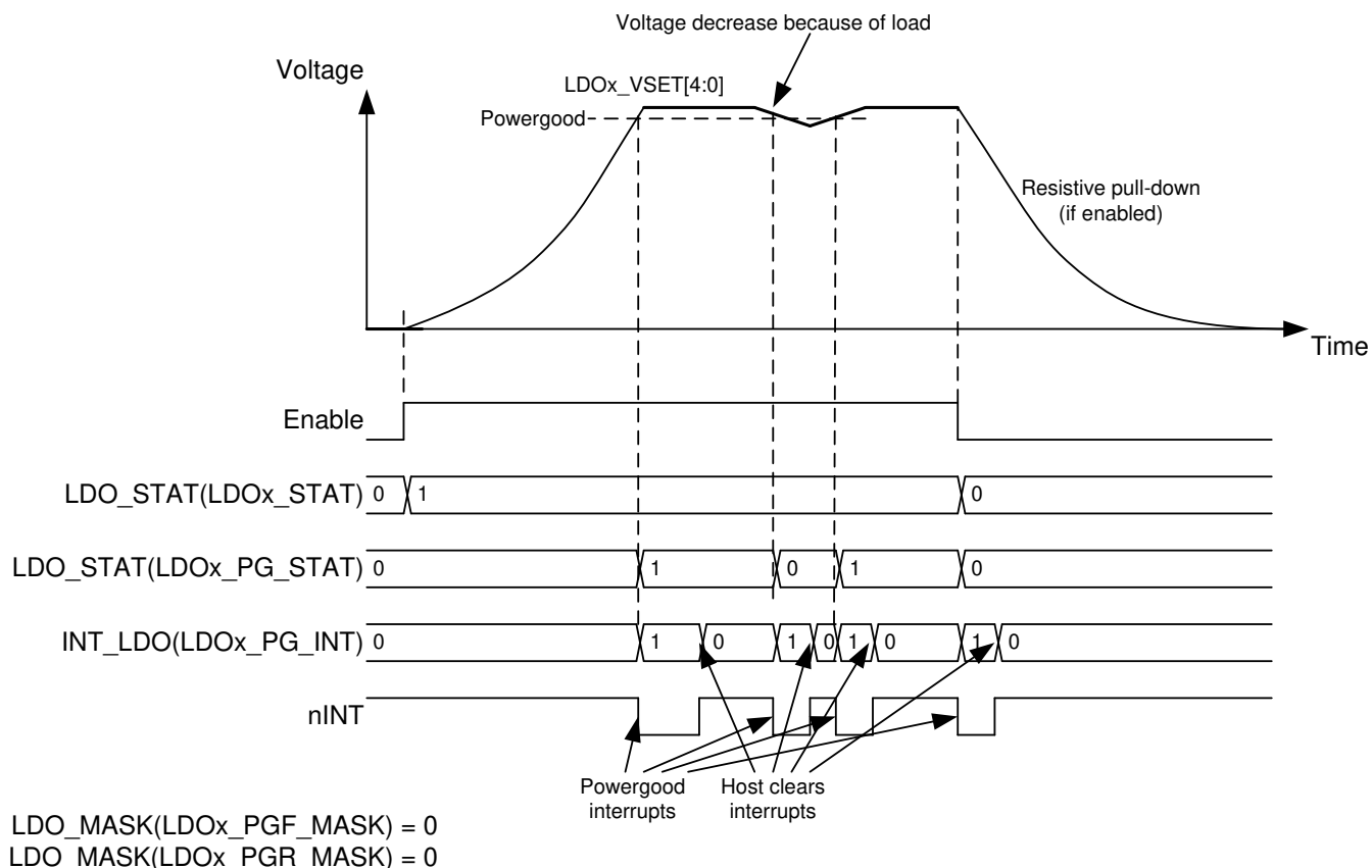
FIG 7-5. LDO Regulator Enable and Disable
