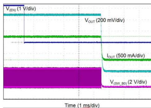
Figure 8-11. Buck Shutdown With EN1, Forced PWM Mode
