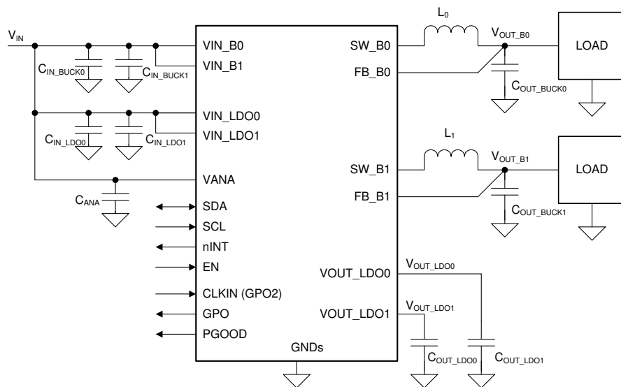
図 8-1. LP87332B-Q1 Typical Application
