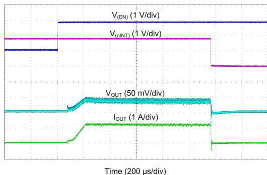
图 8-20. Buck Start-Up With Short on Output
