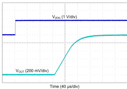
图 8-24. LDO Start-Up
