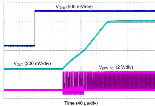
8-9. Buck Start-Up With EN1, Forced PWM Mode
