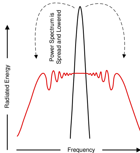
FIG 7-2. Spread-Spectrum Modulation
