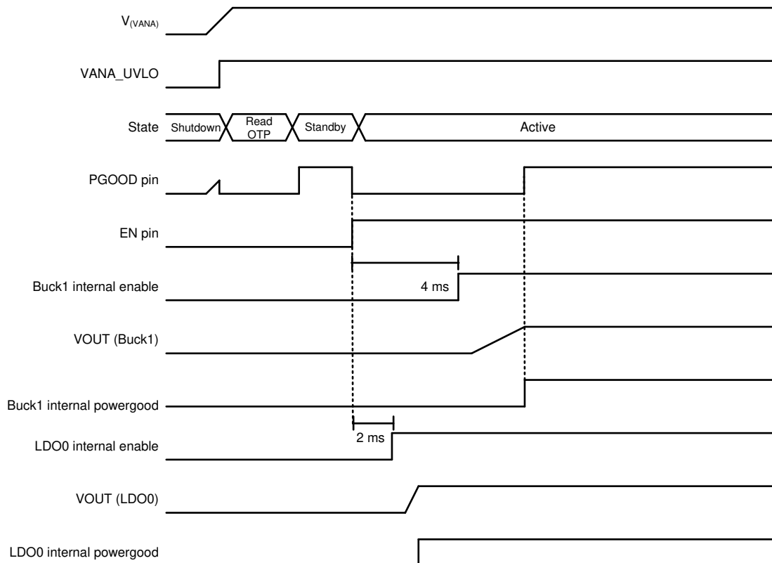
FIG 7-10. PGOOD Pin Operation in Continuous Mode
