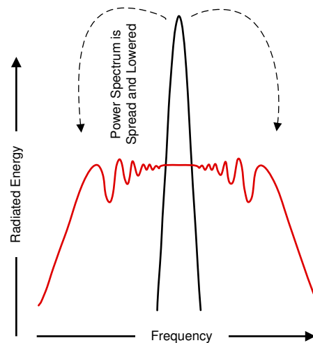
FIG 7-2. Spread-Spectrum Modulation
