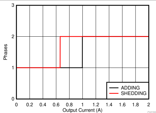
8-17. Buck Phase Adding and Shedding vs Load Current (Dual-Phase Output)
