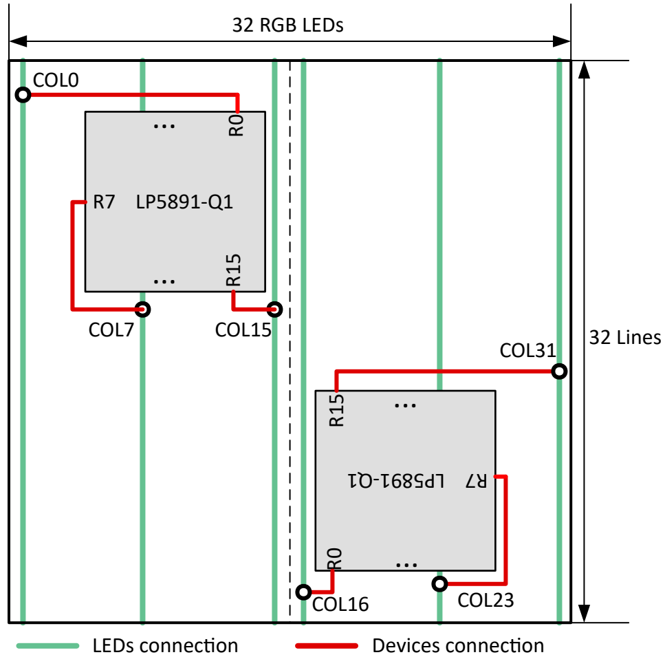
9-12. Channel Routing Suggestion with Channel Order Sequence
