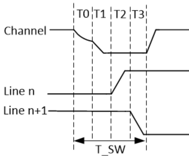
8-7. Line Transitioning Sequence
