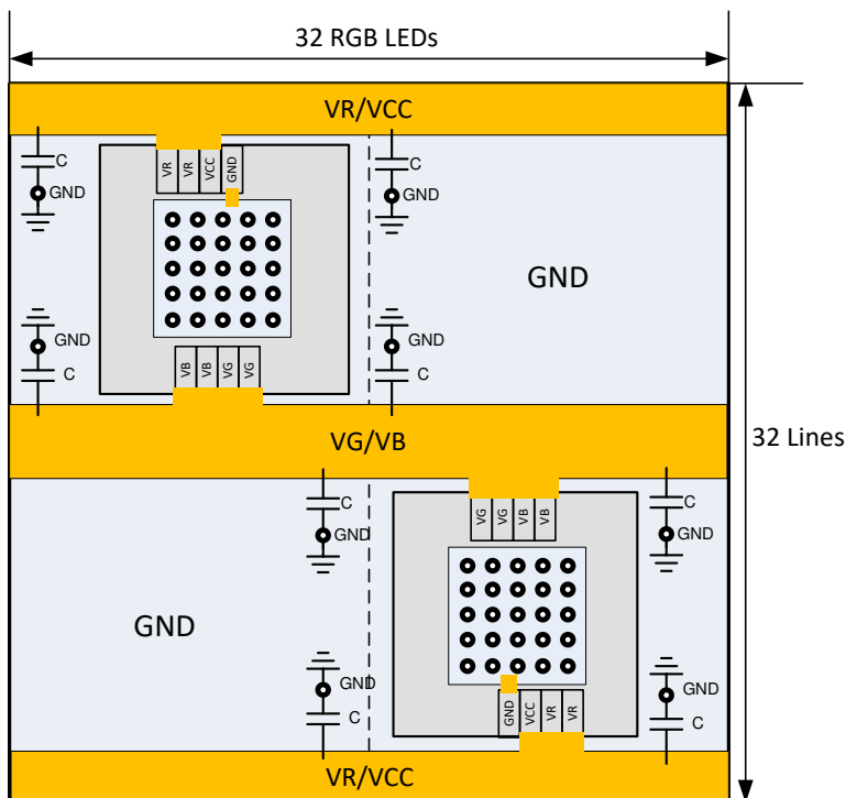
Figure 9-9. Power Rails Routing Suggestion
