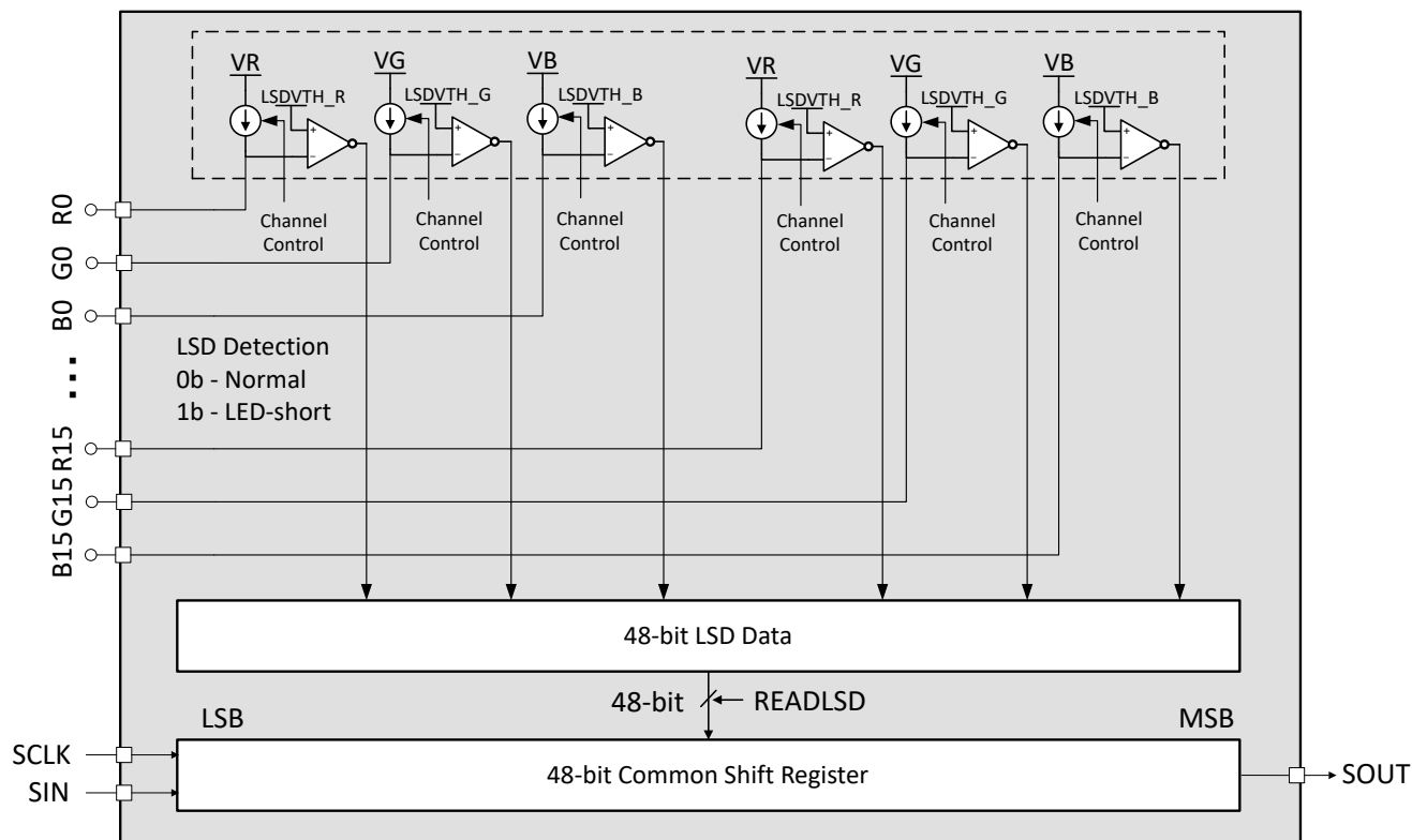
FIG 8-12. LED Short Detection Circuit
