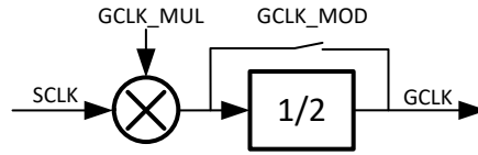
8-6. Frequency Multiplier Block Diagram
