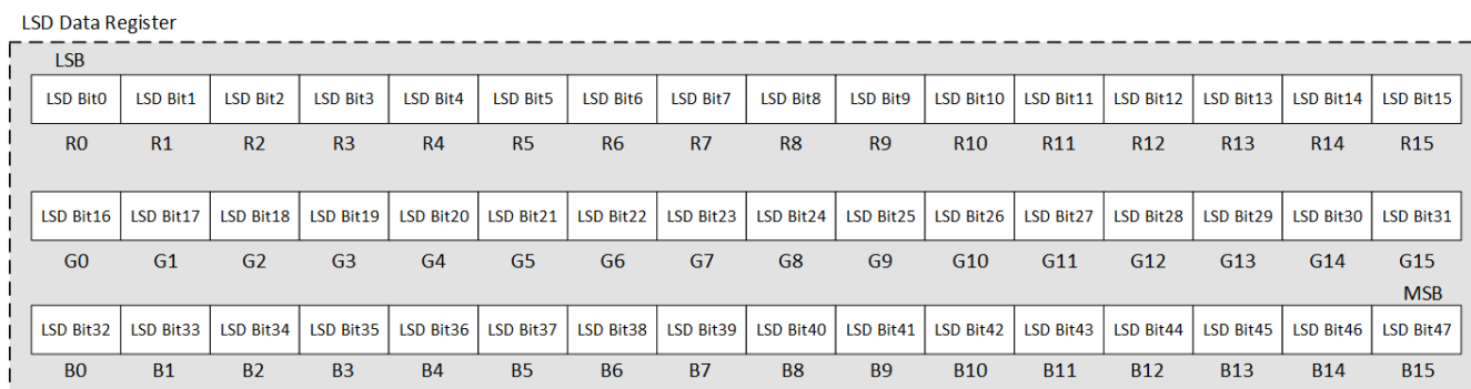
FIG 8-13. Bit Arrangement in the LSD Data Register
