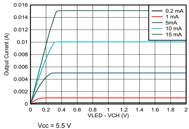
FIG 6-3. Channel Current vs (VLED-Vchannel) Voltage
