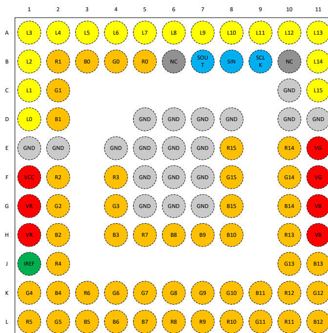
FIG 6-2. LP5890 ZXL Package 96-Pin BGA Top View
