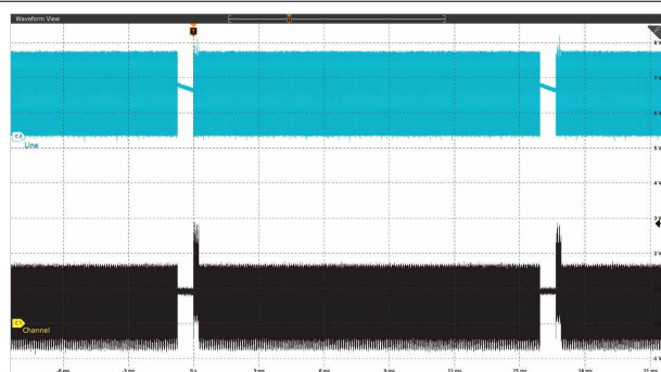
図 9-7. Line and Channel Waveform in One Frame (GSn=0x0001h)
