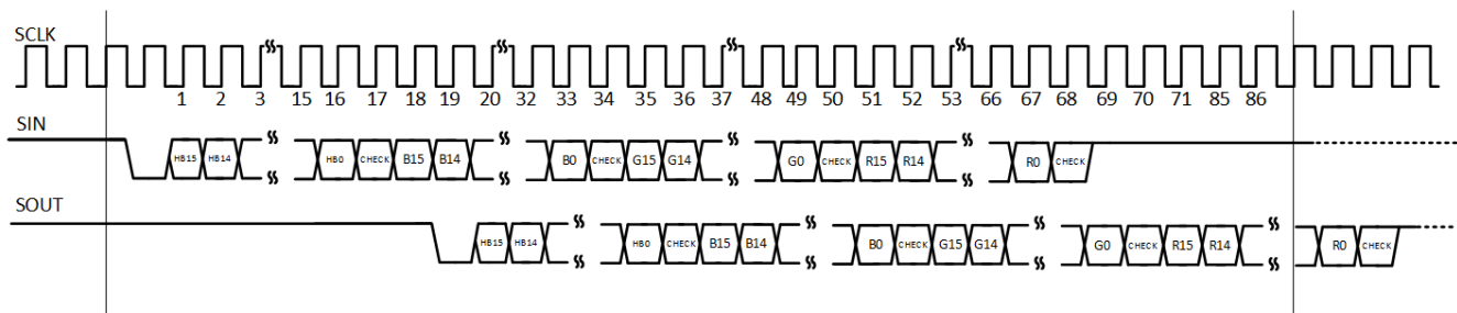
8-18. Data Write Command With Broadcast (Timing Diagram)
