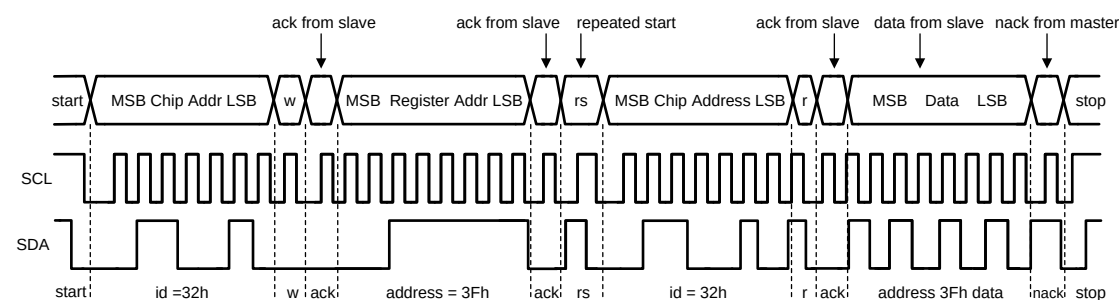
FIG 24. Read Cycle (R = Read; SDA = 1)
