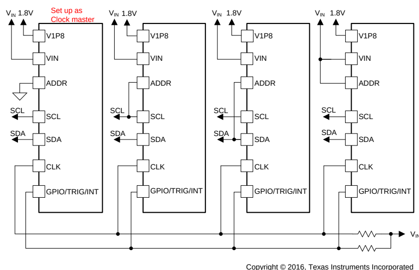
FIG 19. Synchronizing Multiple Devices Using the Clock Generator
