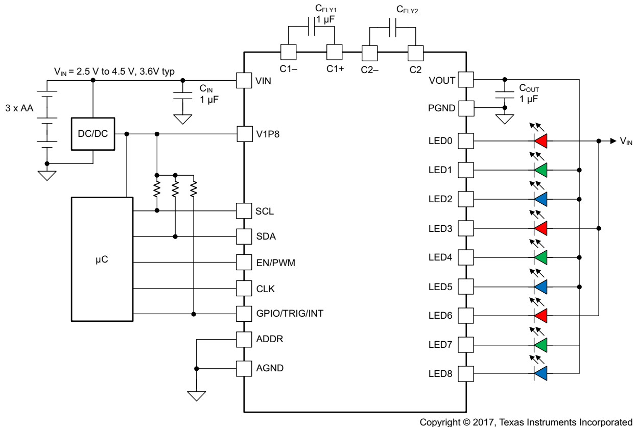
✎ 119. LP5569 Typical Application
