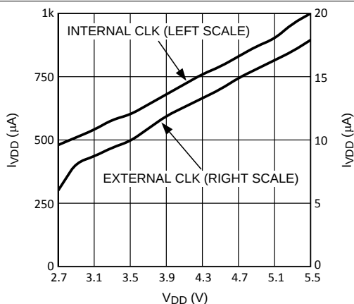
Figure 9. Power Save Mode Supply Current vs V_{DD}
