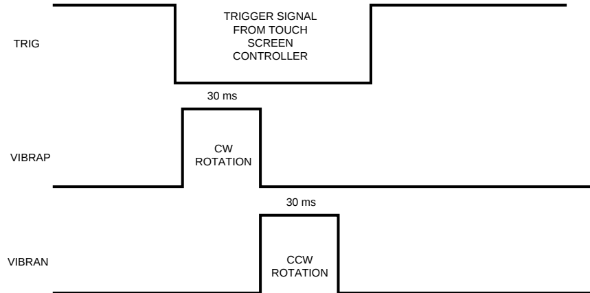
Figure 31. Control Waveform
