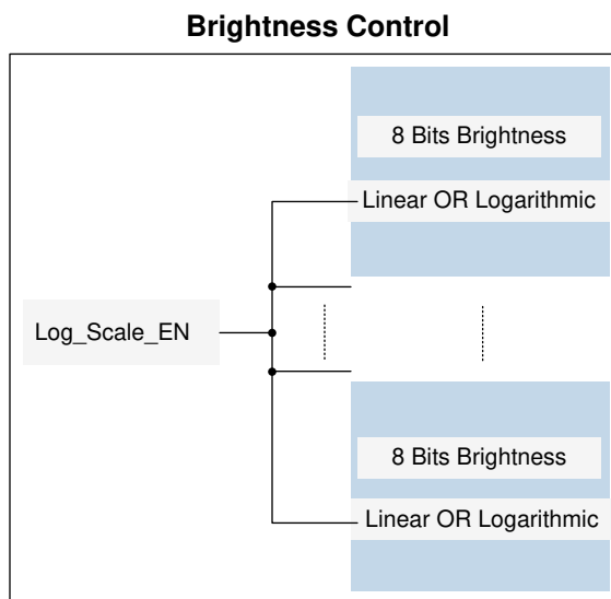
图 8-2. Logarithmic- or Linear-Scale Intensity Control
