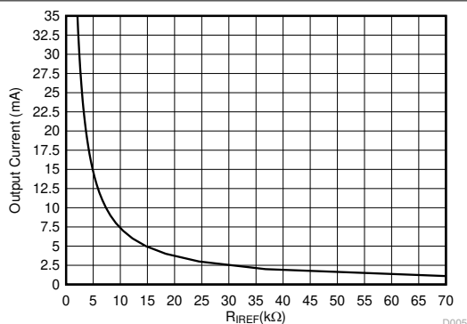
FIG 7-2. I_{OUT} Target vs R_{IREF}
