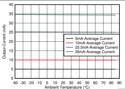
FIG 7-4. Output Current vs Temperature
