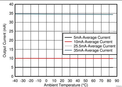
FIG 7-3. Output Current vs Temperature
