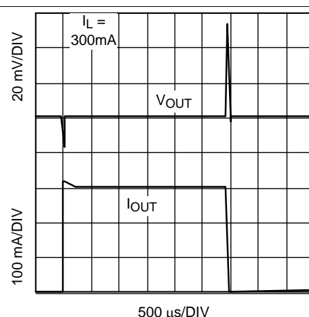
Figure 20. Load Transient
