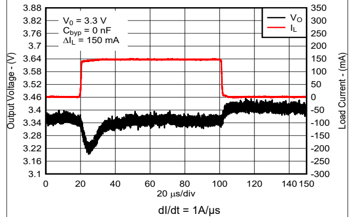
5-40. Load Transient Response (New Chip)
