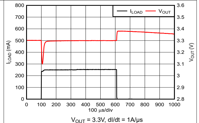
5-42. Load Transient Response (New Chip)
