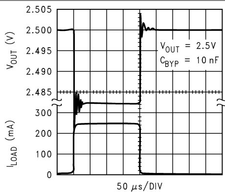
5-39. Load Transient Response (Legacy Chip)
