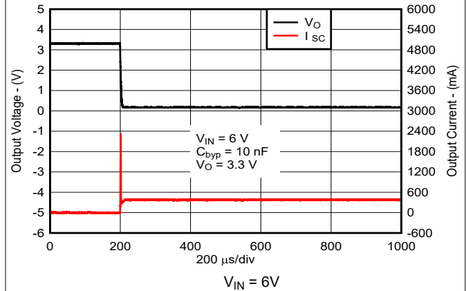
5-4. Short-Circuit Current vs Time (New Chip)
