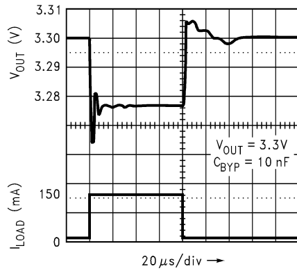
5-37. Load Transient Response (Legacy Chip)
