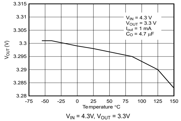
5-2. V_{OUT} vs Temperature (New Chip)
