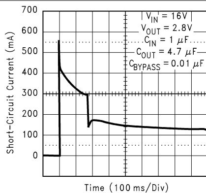
5-3. Short-Circuit Current (Legacy Chip)
