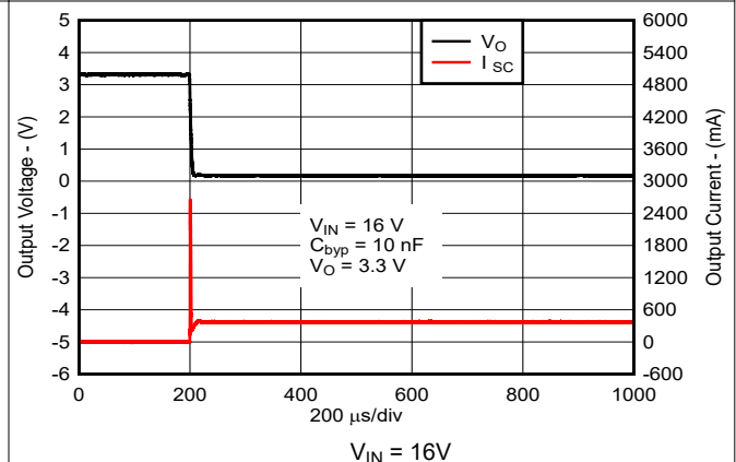
5-6. Short-Circuit Current vs Time (New Chip)
