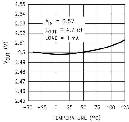
5-1. V_{OUT} vs Temperature (Legacy Chip)
