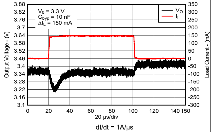
5-38. Load Transient (New Chip)
