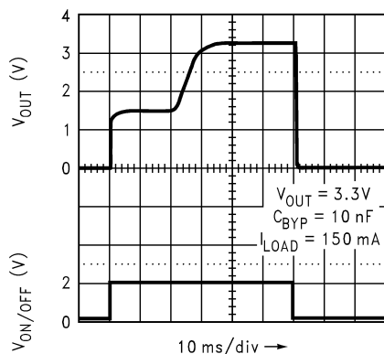
5-55. Turn-On Time (Legacy Chip)
