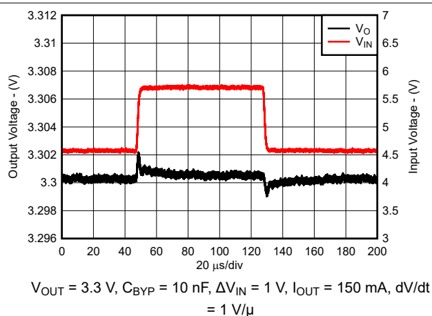
图 7-12. Line Transient Response for New Chip
