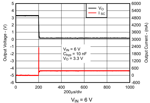
FIG 5-10. Short-Circuit Current vs Time for New Chip
