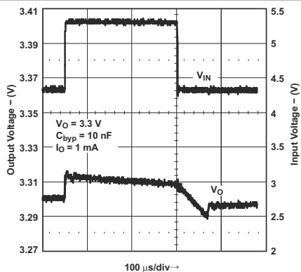
Figure 7-15. Line Transient Response for Legacy Chip
