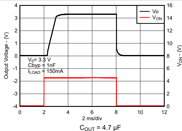
7-22. Turn-On Time for New Chip
