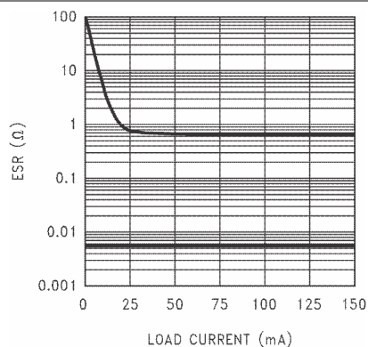
FIG 5-37. 4.7- \mu\text{F} Stable ESR Range for Output Voltage \leq 2.3\text{ V} for Legacy Chip
