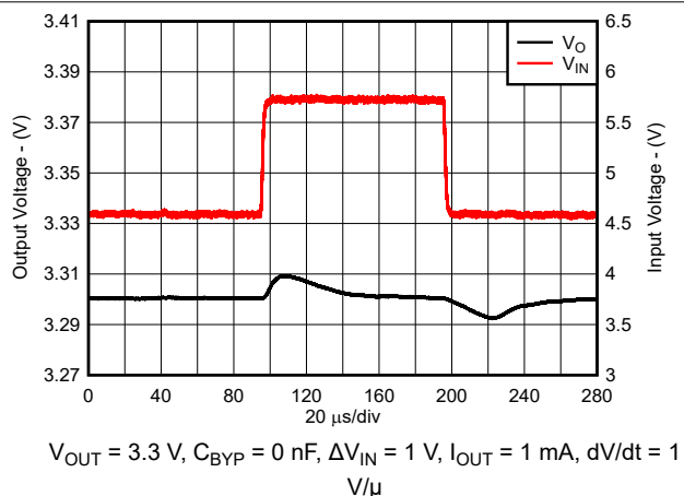
图 7-14. Line Transient Response for New Chip
