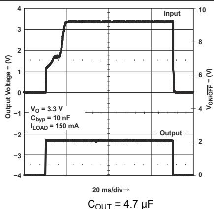
7-23. Turn-On Time
