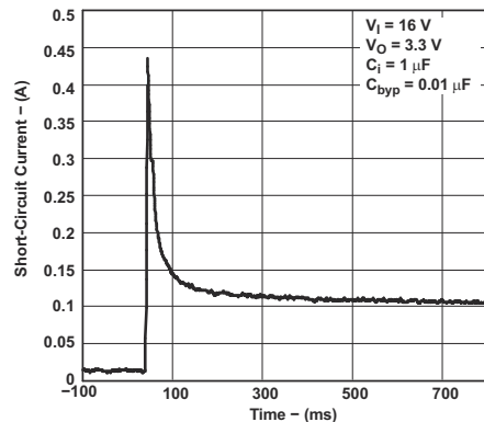
FIG 5-9. Short-Circuit Current vs Time for Legacy Chip
