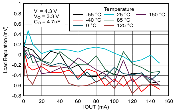
FIG 5-7. Output Regulation vs Load Current for New Chip
