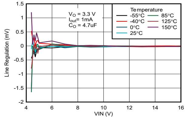
FIG 5-8. Output Regulation vs Input Voltage for New Chip
