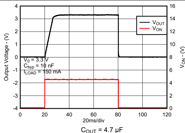
7-24. Turn-On Time for New Chip
