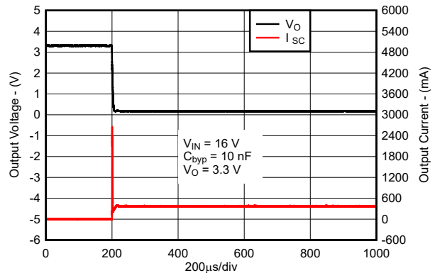
FIG 5-10. Short-Circuit Current vs Time for New Chip
