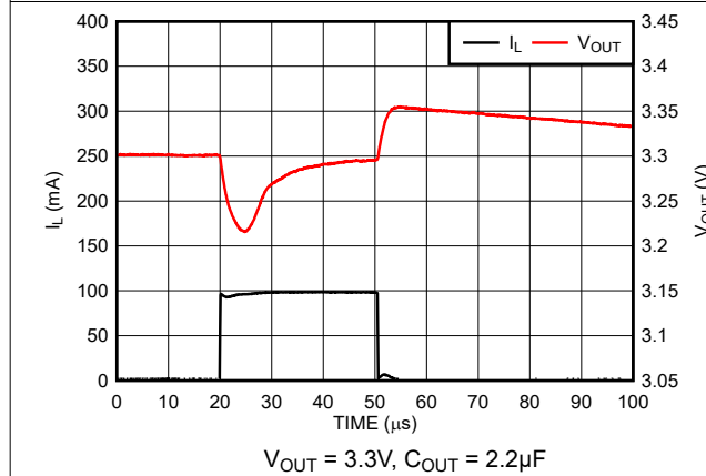
Figure 5-15. Load Transient Response (New Chip)
