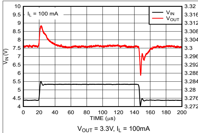
Figure 5-13. Line Transient Response (New Chip)
