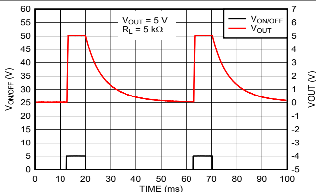
图 5-26. Turn-Off Waveform (New Chip)
