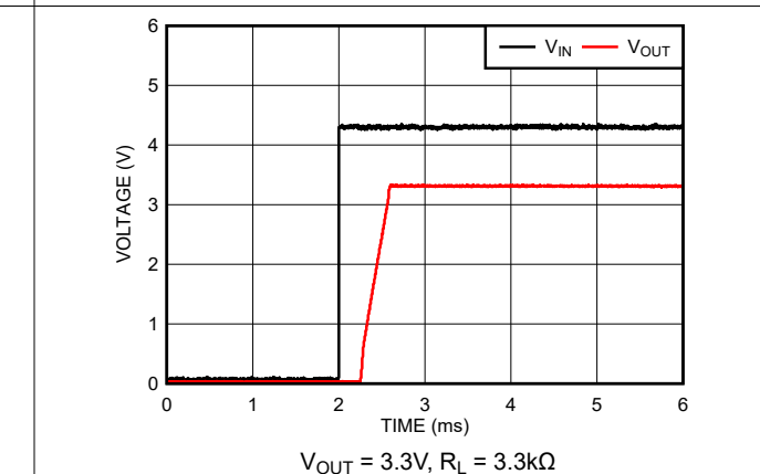
Figure 7-10. Turn-On Waveform (New Chip)
