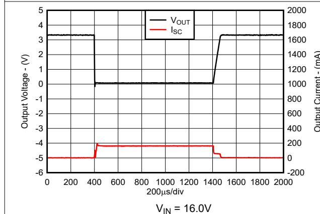
Figure 5-17. Short-Circuit Current vs Time (New Chip)
