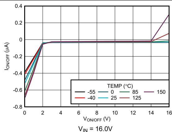
图 5-28. ON/OFF Pin Current vs V ON/OFF (New Chip)
