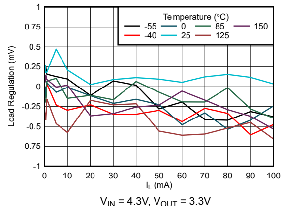
Figure 5-3. Load Regulation vs Temperature (New Chip)
