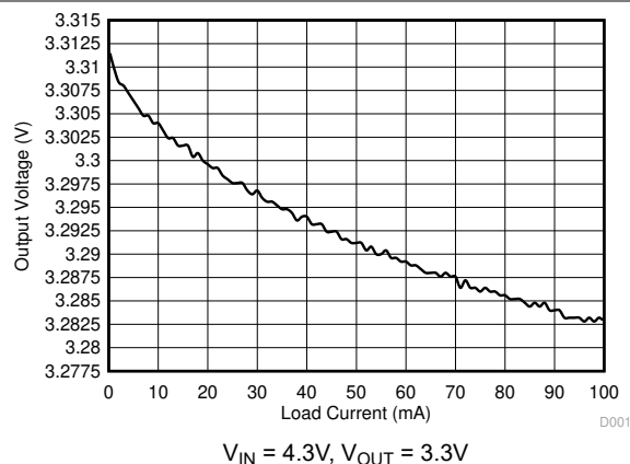
Figure 5-1. Output Voltage vs Load Current (Legacy Chip)
