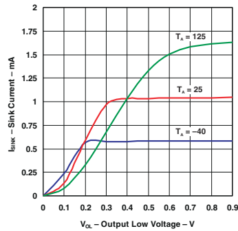
FIG 5-33. LP2951 ERROR Comparator Sink Current vs Output Low Voltage (Legacy Chip)
