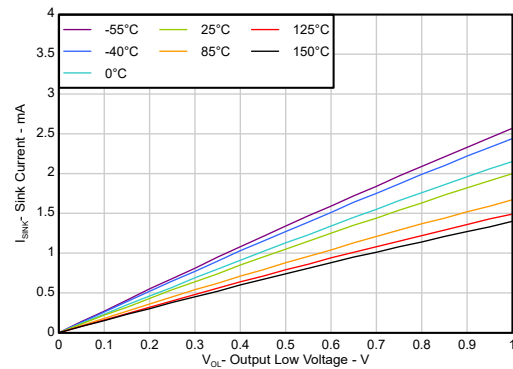
FIG 5-34. ERROR Comparator Sink Current vs Output Low Voltage (New Chip)
