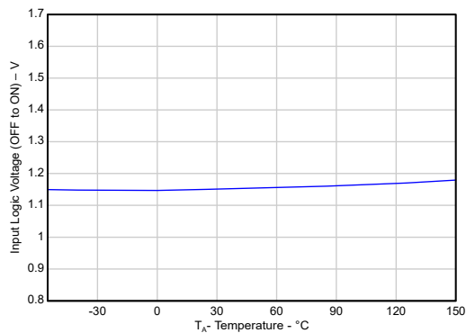
FIG 5-37. Shutdown Threshold Voltage (Off to On) vs Temperature (New Chip)
