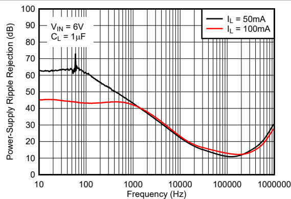
Figure 5-57. Ripple Rejection vs Frequency (Legacy Chip)
