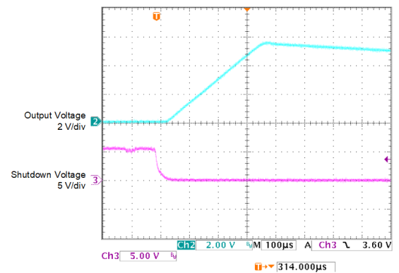
✎ 5-52. Enable Transient Response vs Time ( I_L = 1\text{mA} , C_L = 10\mu\text{F} )
