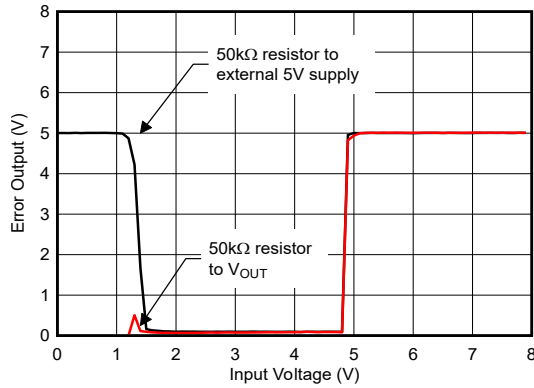
FIG 5-31. LP2951 ERROR Comparator Output vs Input Voltage (Legacy Chip)
