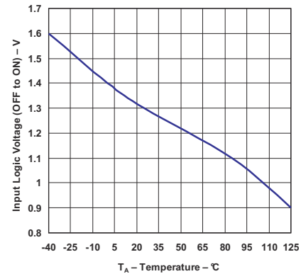
FIG 5-36. Shutdown Threshold Voltage (Off to On) vs Temperature (Legacy Chip)
