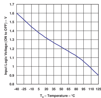
FIG 5-38. Shutdown Threshold Voltage (On to Off) vs Temperature (Legacy Chip)
