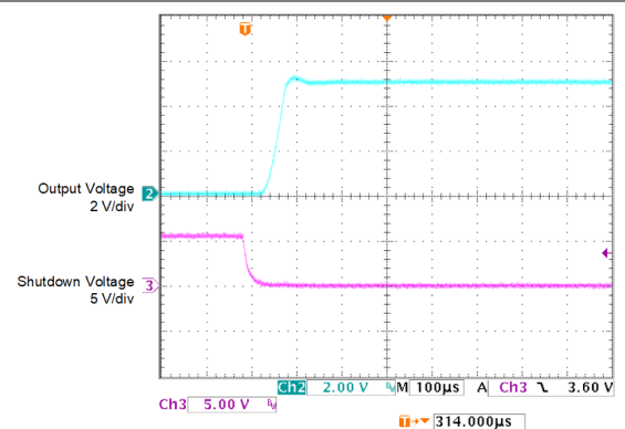
✎ 5-50. Enable Transient Response vs Time ( I_L = 1\text{mA} , C_L = 1\mu\text{F} ) (Legacy Chip)
