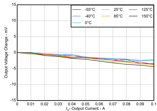
FIG 5-42. Load Regulation vs Load Current (New Chip)
