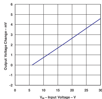
FIG 5-40. Line Regulation vs Input Voltage (Legacy Chip)
