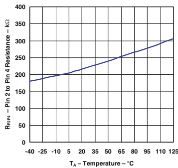
FIG 5-35. LP2951 Divider Resistance vs Temperature (Legacy Chip)
