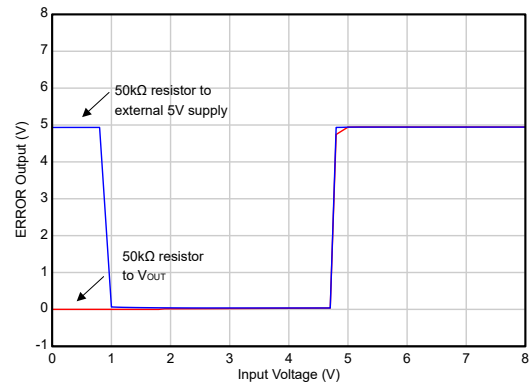
FIG 5-32. ERROR Comparator Output vs Input Voltage (New Chip)
