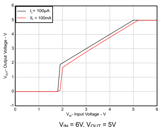
5-43. Output Voltage vs Input Voltage (New Chip)
