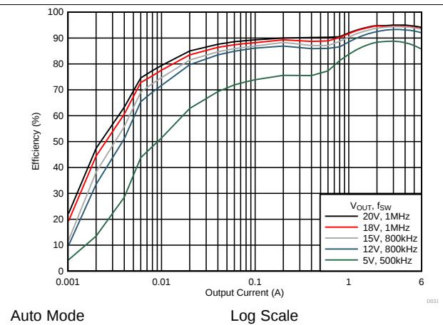
FIG 24. Efficiency vs Output Current
