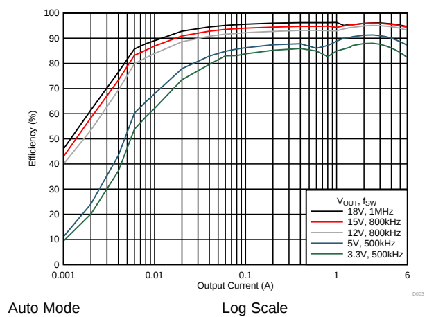
FIG 14. Efficiency vs Output Current
