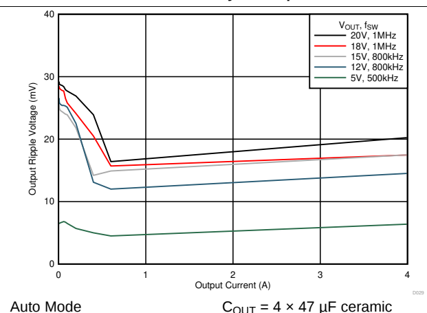
FIG 26. Output Voltage Ripple
