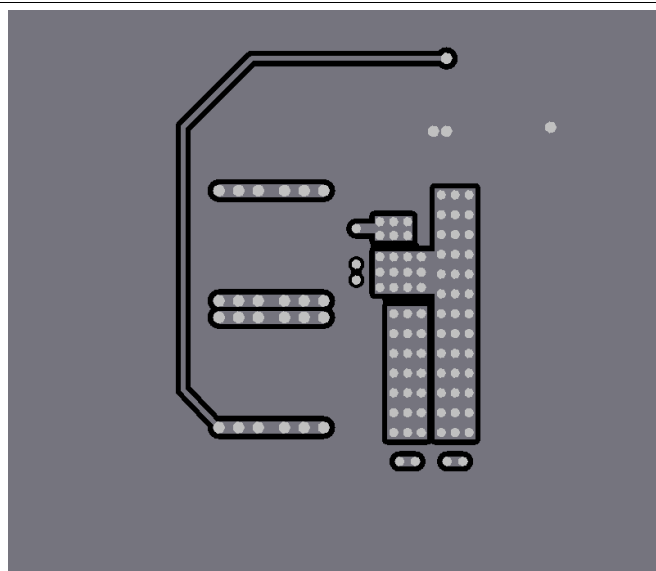
Figure 51. Typical Bottom-Layer Layout
