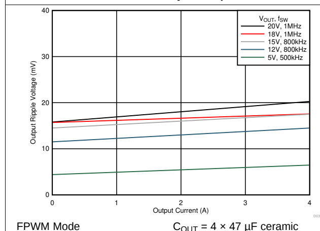
FIG 25. Output Voltage Ripple
