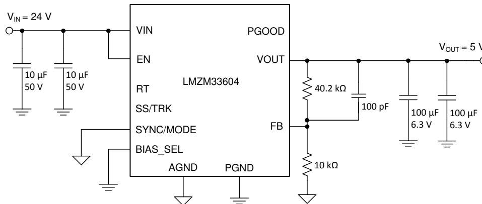
図 45. LMZM33604 Typical Schematic
