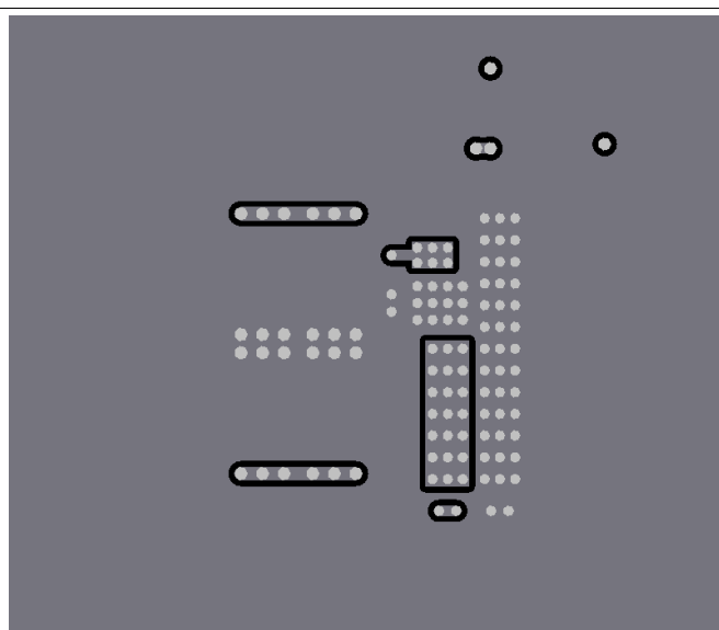
Figure 49. Typical Layer-2 Layout
