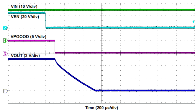
Figure 30. Enable Turn-OFF
