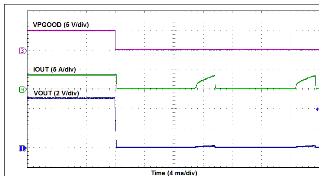
7-15. Overcurrent Limiting
