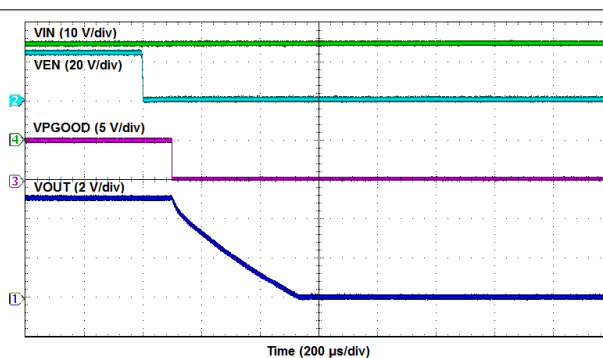
Figure 7-12. Enable Turn-OFF
