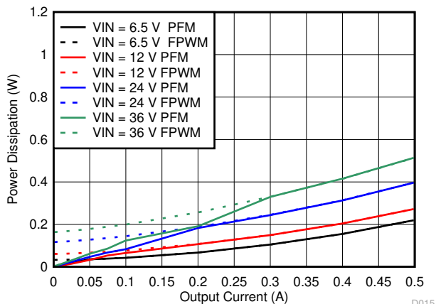
Figure 7-9. Power Dissipation
