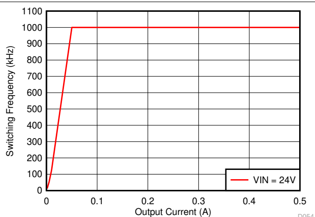
7-27. Auto PFM Mode Switching Frequency vs Output Current
