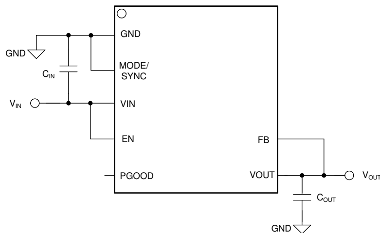
図 9-1. Fixed 5-V or 3.3-V Typical Application Circuit
