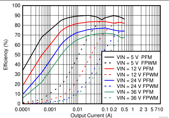
Figure 9-30. Efficiency
