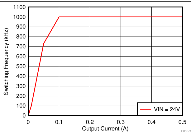
7-26. Auto PFM Mode Switching Frequency vs Output Current
