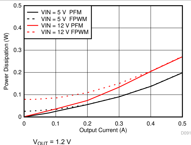
7-15. Power Dissipation
