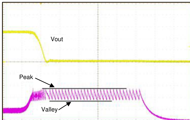
图 8-1. Current Limit Operation During Output Short Circuit
