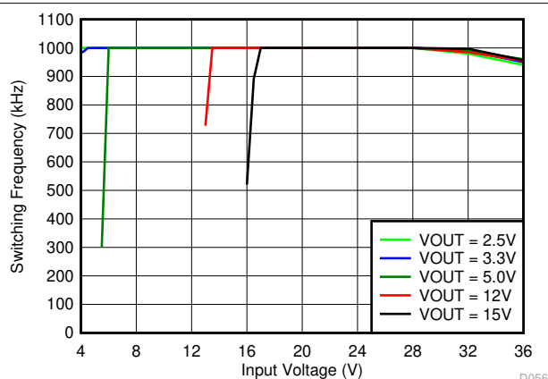
7-30. Switching Frequency vs Input Voltage for Adjustable Output Options at Full Load
