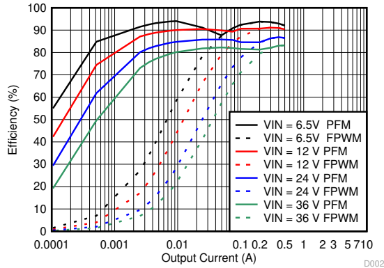
9-6. Efficiency
