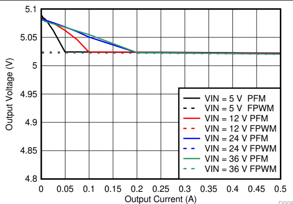
9-10. Line and Load Regulation
