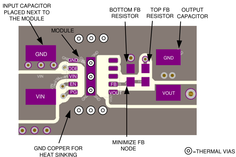
9-50. Layout Example With Adjustable Output Version
