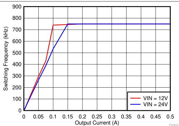
7-25. Auto PFM Mode Switching Frequency vs Output Current
