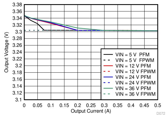
Figure 9-45. Line and Load Regulation for V_{OUT} = 3.3\text{ V}
