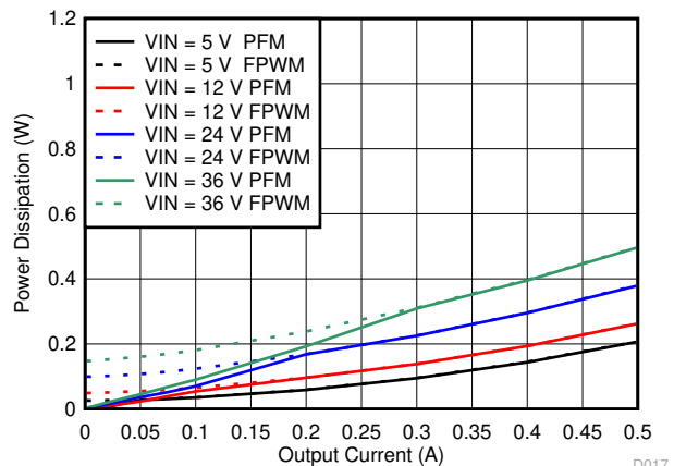
Figure 7-10. Power Dissipation
