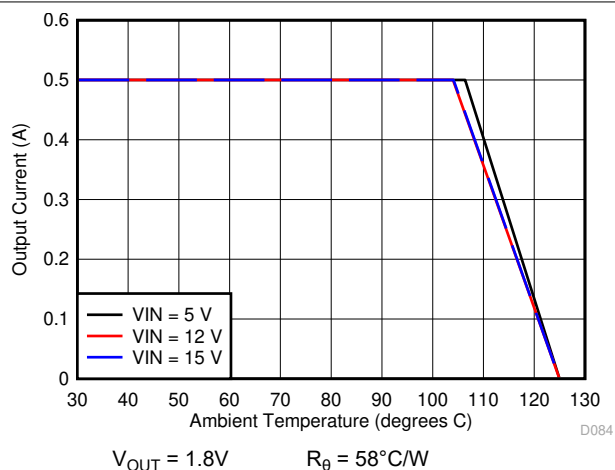
7-17. Ambient Temperature vs Output Current
