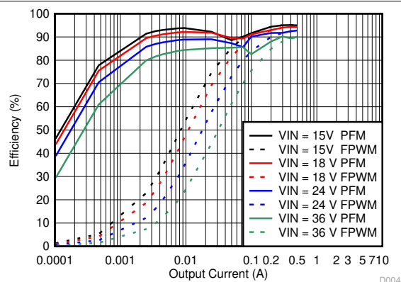
9-18. Efficiency
