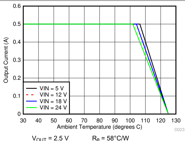
7-18. Ambient Temperature vs Output Current
