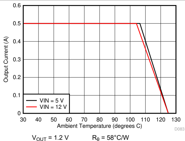
7-16. Ambient Temperature vs Output Current
