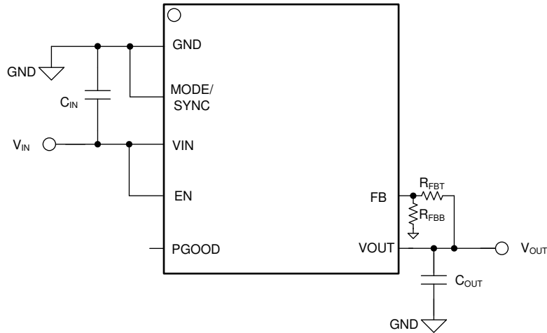
図 9-4. Adjustable 1.2-V to 15-V Output Typical Application Circuit
