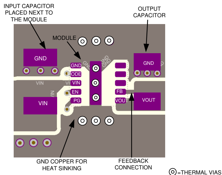
FIG 9-49. Layout Example With Fixed Output Version
