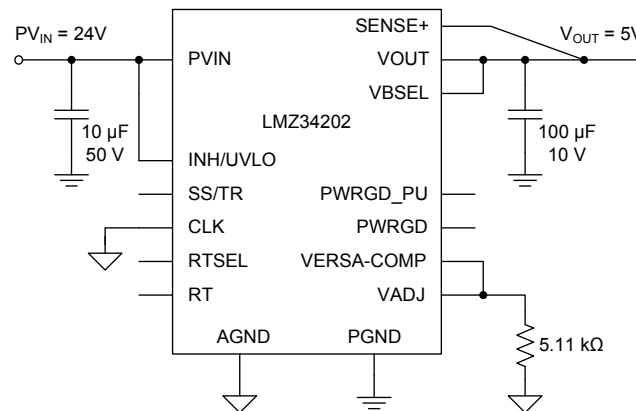
図 27. LMZ34202 Minimum External Component Application
