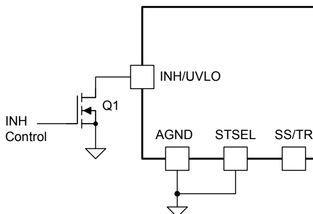
Figure 26. Typical Inhibit Control
