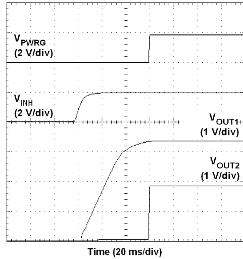
Figure 36. Sequencing Waveforms
