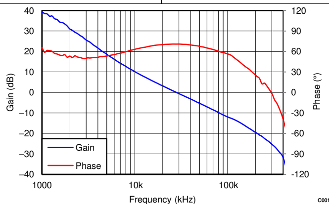
Figure 5. V OUT = 1.8 V, I OUT = 4 A, C OUT = 200 μF Ceramic, f sw = 500 kHz
