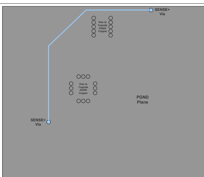
Figure 37. Typical PGND-Layer Recommended Layout
