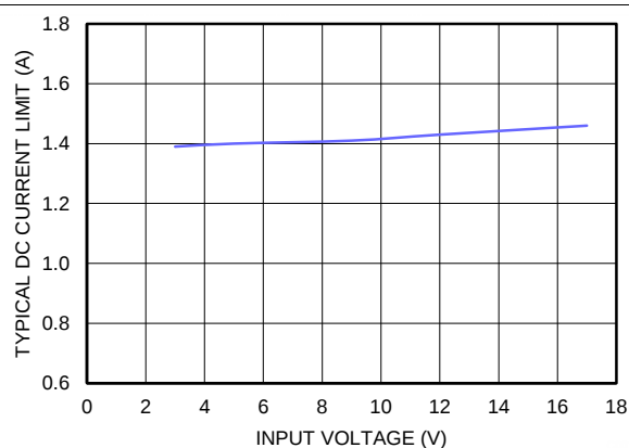
Figure 29. Typical Current Limit V_{OUT} = 1.2 V, T_A = 85^\circ\text{C}
