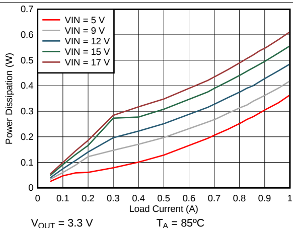
Figure 4. Power Dissipation
