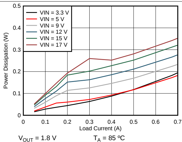
Figure 4. Power Dissipation
