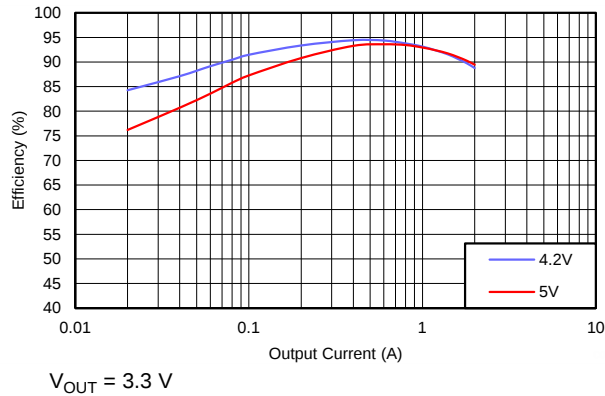
Figure 32. Efficiency
