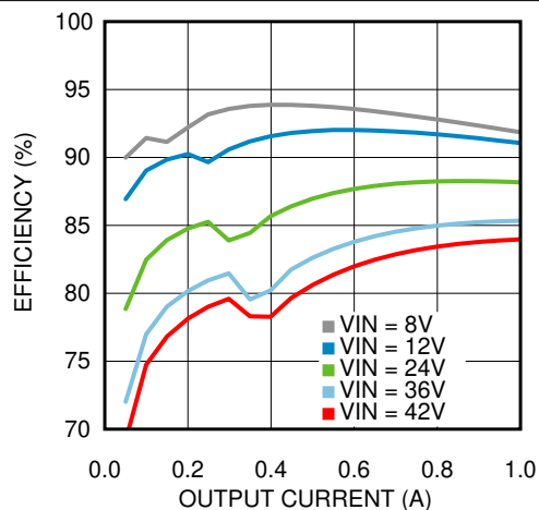
FIG 6-13. Efficiency V_{OUT} = 5\text{ V} , T_A = 85^\circ\text{C}
