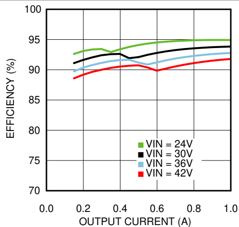
FIG 6-17. Efficiency V_{OUT} = 15\text{ V} , T_A = 85^\circ\text{C}
