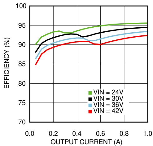
FIG 6-5. Efficiency V_{OUT} = 15\text{ V} , T_A = 25^\circ\text{C}
