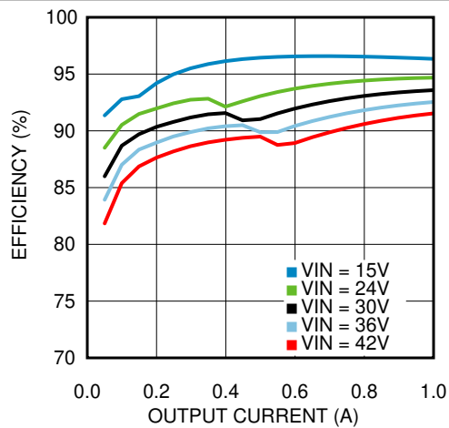
FIG 6-3. Efficiency V_{OUT} = 12\text{ V} , T_A = 25^\circ\text{C}
