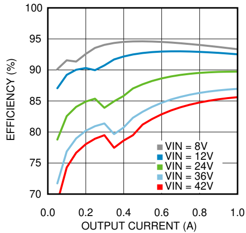
FIG 6-1. Efficiency V_{OUT} = 5\text{ V} , T_A = 25^\circ\text{C}
