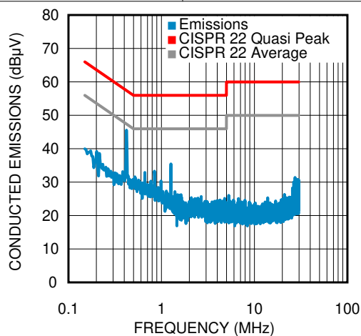
6-45. Conducted EMI, V_{OUT} = 12\text{ V} Evaluation Board BOM and 3.3\text{-}\mu\text{H} , 1\text{-}\mu\text{F} LC Line Filter
