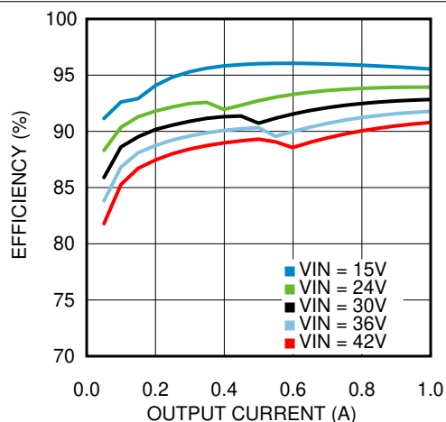
FIG 6-15. Efficiency V_{OUT} = 12\text{ V} , T_A = 85^\circ\text{C}
