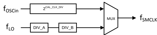
✎ 49. Block Diagram of SM Clock
