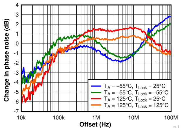
图 6-14. Change in VCO Phase Noise Over Temperature
