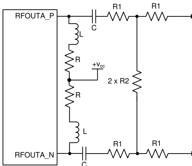
FIG 8-7. Termination of Unused Output - Differential
