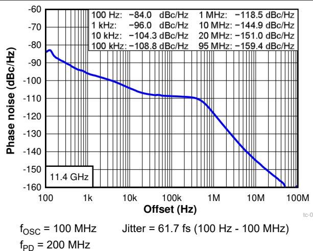
图 6-7. Closed Loop Phase Noise at 11.4 GHz
