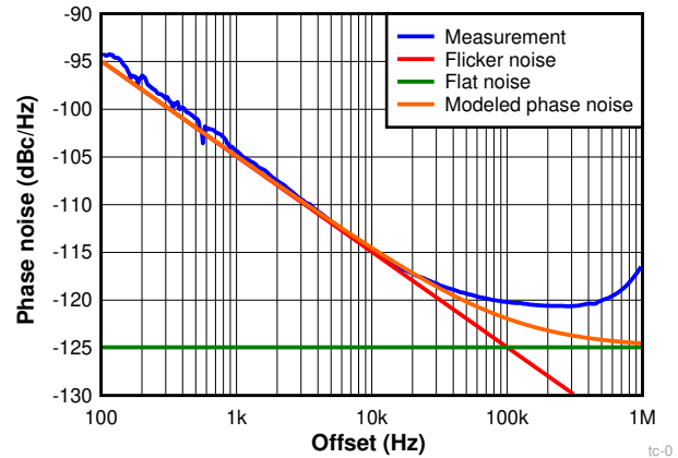
FIG 6-11. Calculation of PLL Noise Metrics
