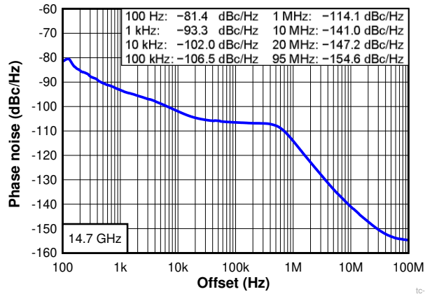
FIG 6-10. Closed Loop Phase Noise at 14.7 GHz
