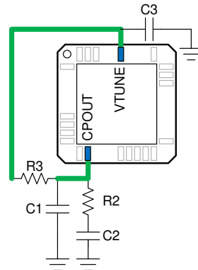
FIG 8-8. External Loop Filter
