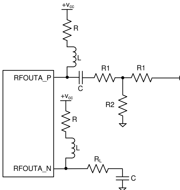
FIG 8-6. Termination of Unused Output - Single-Ended
