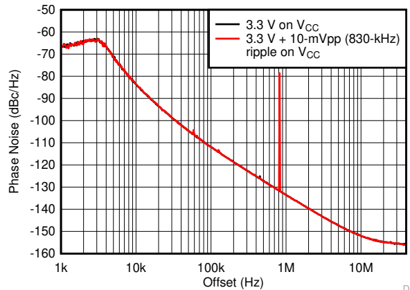
FIG 6-11. Impact of Supply Ripple on 6-GHz Output Phase Noise
