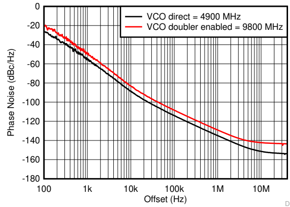
FIG 6-7. 9.8-GHz Output - Open-Loop Phase Noise
