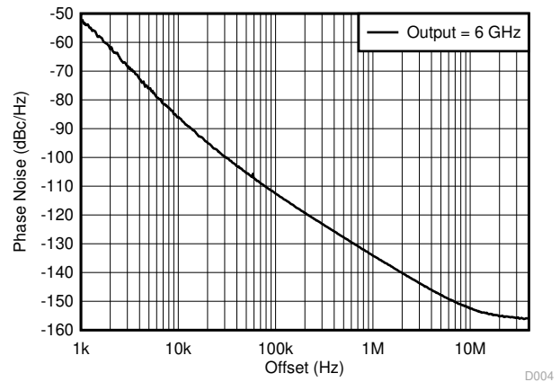
FIG 6-5. 6-GHz Output - Open-Loop Phase Noise
