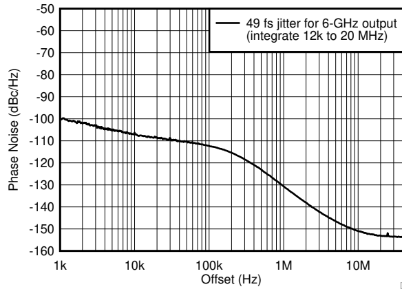
FIG 6-8. Integrated Jitter (49 fs) - 6-GHz Output
