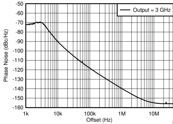
FIG 6-2. 3-GHz Output - Closed-Loop Phase Noise
