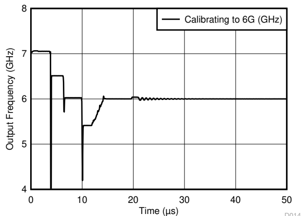
FIG 6-15. 20- \mu\text{s} Frequency Change Time to 6 GHz With Fast Calibration
