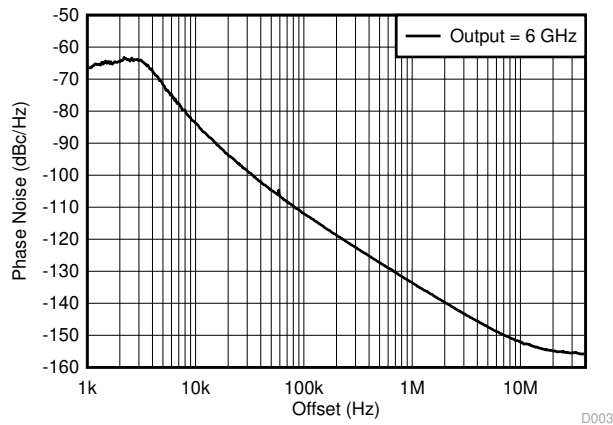
FIG 6-4. 6-GHz Output - Closed-Loop Phase Noise
