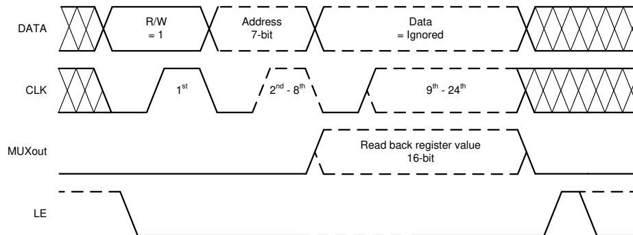
FIG 7-4. Register Readback Timing Diagram
