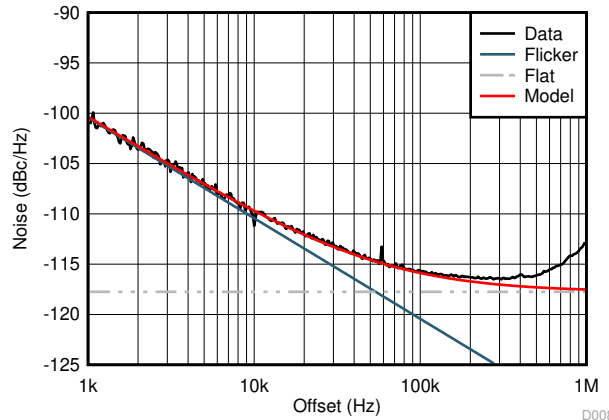
FIG 6-9. 6-GHz Output Wide Loop Bandwidth – Showing PLL Performance
