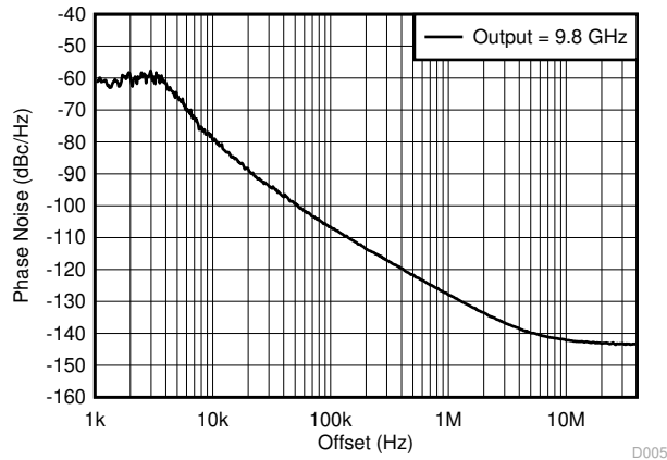
FIG 6-6. 9.8-GHz Output - Closed-Loop Phase Noise
