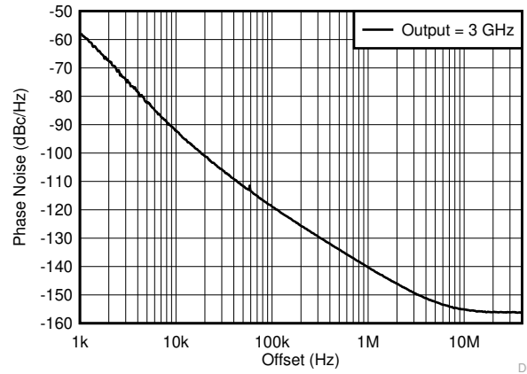
FIG 6-3. 3-GHz Output - Open-Loop Phase Noise
