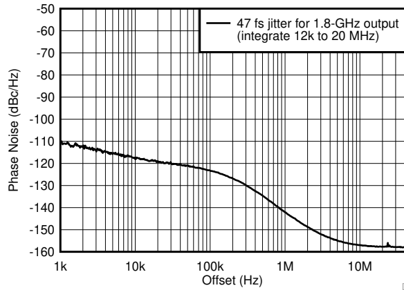
FIG 6-8. Integrated Jitter (47 fs) - 1.8-GHz Output
