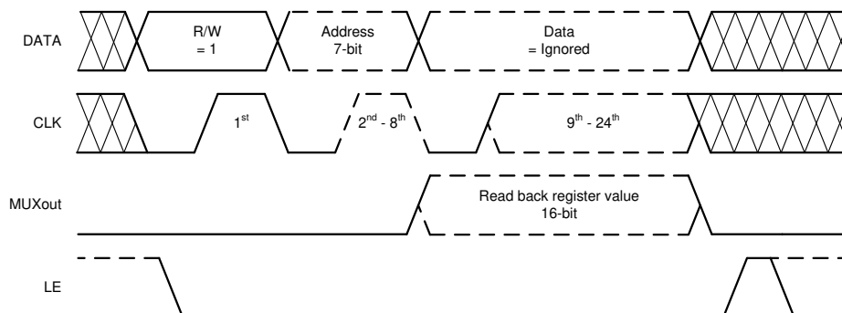
7-4. Register Readback Timing Diagram
