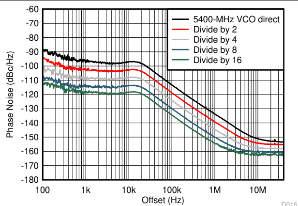
FIG 6-16. Impact of Channel Divider Settings on Phase Noise
