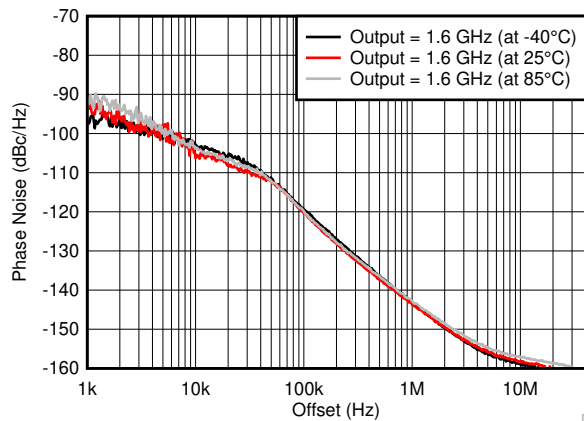
FIG 6-10. Variation of Phase Noise Across Temperature
