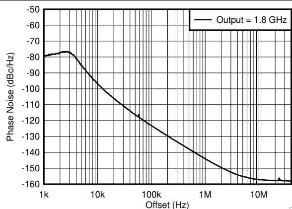
FIG 6-4. 1.8-GHz Output - Closed-Loop Phase Noise
