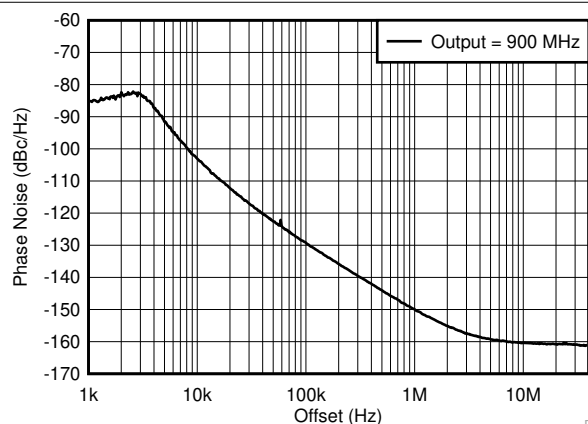
FIG 6-2. 900-MHz Output - Closed-Loop Phase Noise
