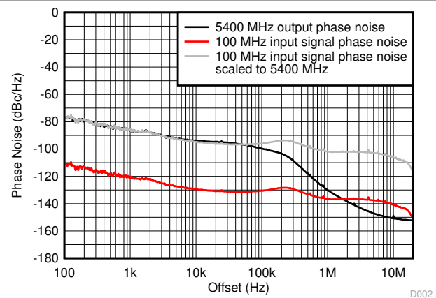
8-3. Phase Noise of 5.4-GHz Output With High-Noise Input Signal
