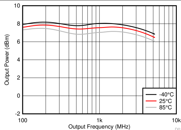
FIG 6-12. High Output Power (50-Ω Pullup, Single-Ended) vs Output Frequency
