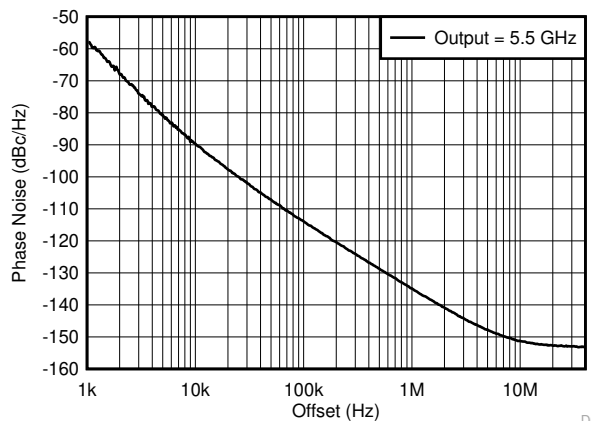
FIG 6-7. 5.5-GHz Output - Open-Loop Phase Noise
