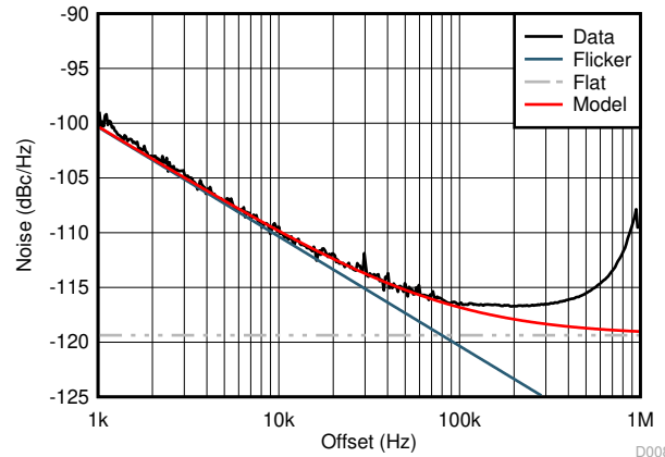
FIG 6-9. 5.4-GHz Output Wide Loop Bandwidth – Showing PLL Performance
