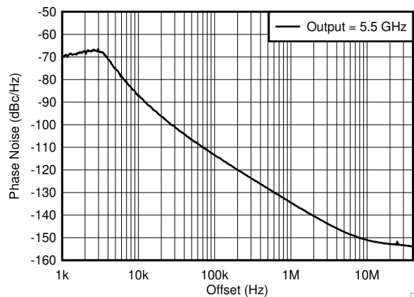
FIG 6-6. 5.5-GHz Output - Closed-Loop Phase Noise
