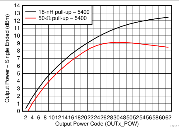
FIG 6-13. Output Power at 5.4-GHz Output vs OUTx_POW Code (1 - 31, 48 - 63)
