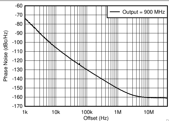
FIG 6-3. 900-MHz Output - Open-Loop Phase Noise
