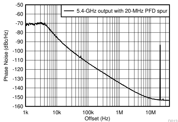
FIG 6-14. Typical PFD Spur for 5.4-GHz Output
