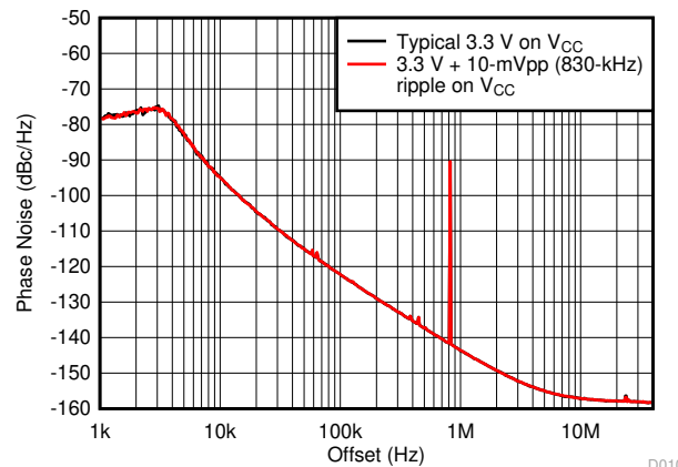
FIG 6-11. Impact of Supply Ripple on 1.8-GHz Output Phase Noise
