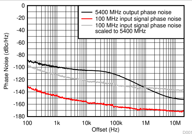
8-2. Phase Noise of 5.4-GHz Output With Low-Noise Input Signal
