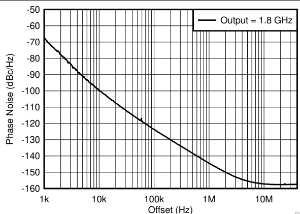
FIG 6-5. 1.8-GHz Output - Open-Loop Phase Noise
