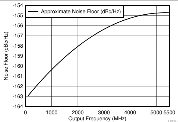
FIG 6-17. Noise Floor Variation With Output Frequency
