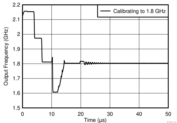
FIG 6-15. 20-μs Frequency Change Time to 1.8 GHz With Fast Calibration
