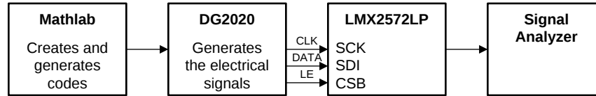
✎ 170. Application Example Test Setup
