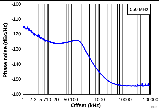
图 11. Wide Band Phase Noise at 550 MHz
