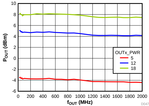
FIG 155. Output Power vs Frequency
