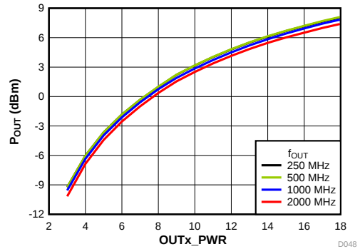
FIG 156. Output Power vs Power Control Bits
