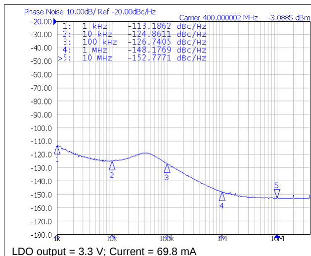
☒ 175. Phase Noise With LDO Power Supply
