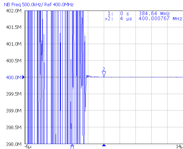
FIG 157. Buffer Power Up at 400-MHz Output
