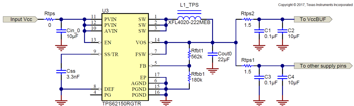
174. Power Supply With a DC/DC Converter
