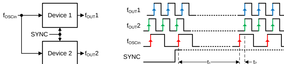
FIG 23. Phase Synchronization
