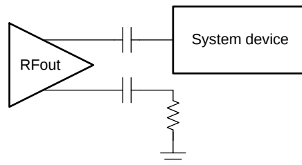
FIG 158. Unused Output Buffer Differential Pin
