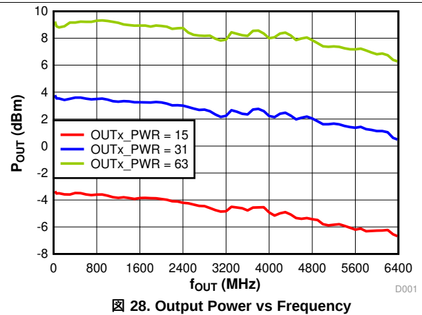
Figure 28. Output Power vs Frequency
