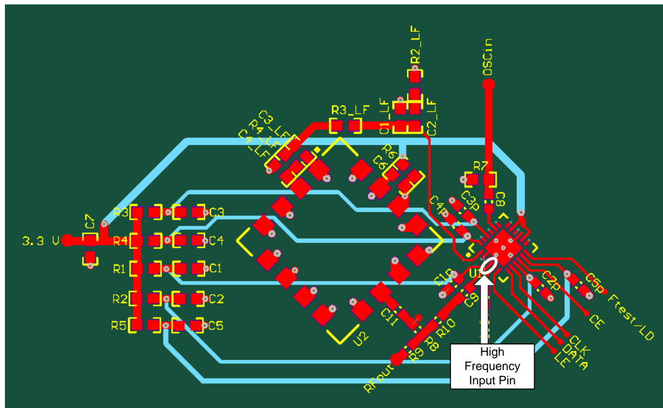
Figure 36. Layout Example
