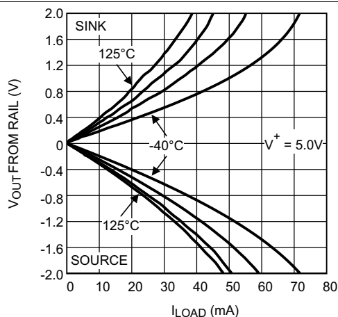
Figure 22. Output Voltage Swing vs Load Current at V^+ = 5.0\text{ V}
