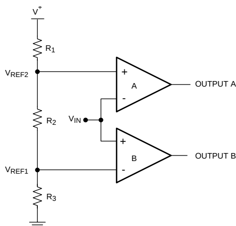
Figure 29. Window Detector
