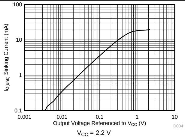
FIG 4. Sinking Current vs Output Voltage
