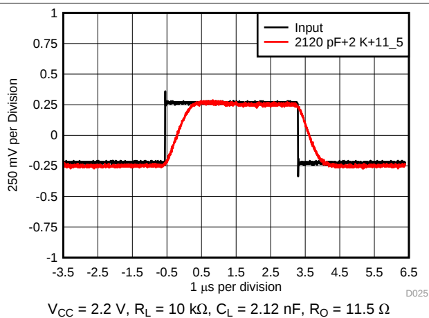
⊠ 25. Pulse Response
