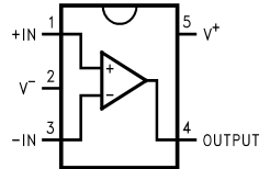
LMV651 DBV or DCK Package 5-Pin SC70 or SOT-23 Top View
