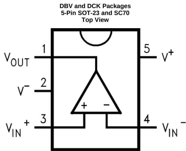
Pin Functions
