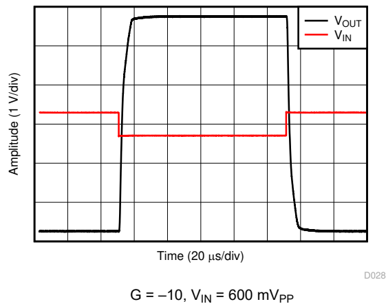
Figure 6-23. Overload Recovery
