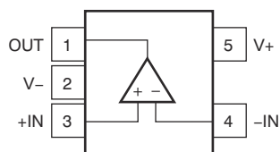
図 5-1. LMV321A-Q1 DBV Package, 5-Pin SOT-23 (Top View)
