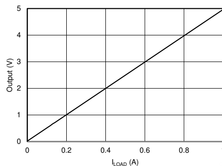
図 8-2. Low-Side, Current-Sense Transfer Function
