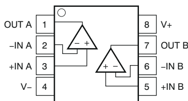
図 5-3. LMV358A-Q1 D and DGK Packages, 8-Pin SOIC and VSSOP (Top View)
