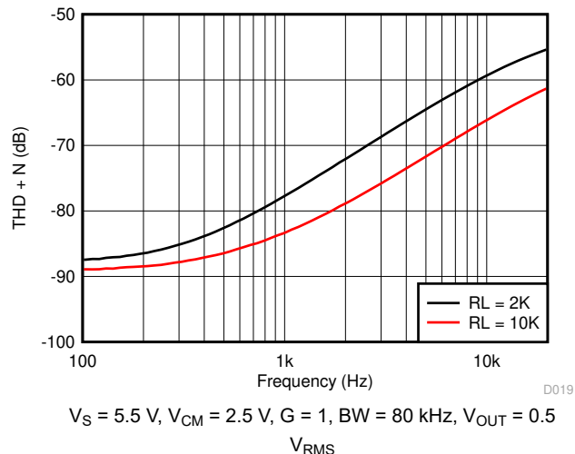
6-14. THD + N vs Frequency
