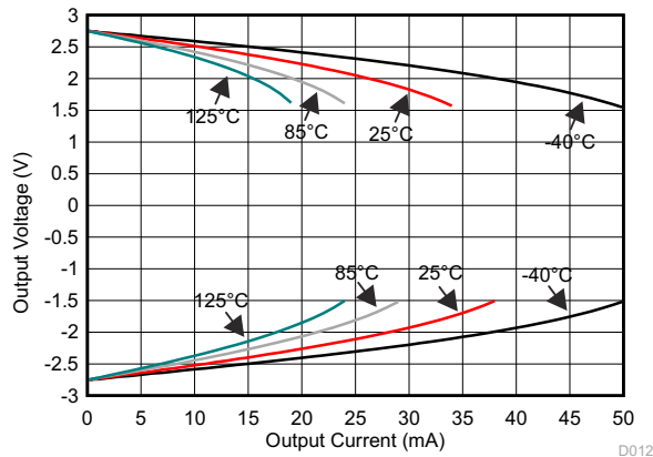
6-7. Output Voltage vs Output Current (Claw)
