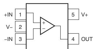
図 5-2. LMV321A-Q1 DCK, LMV321AU-Q1 DBV Package, 5-Pin SC70, SOT-23 (Top View)
