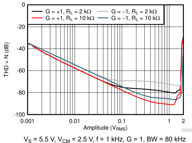
6-15. THD + N vs Amplitude
