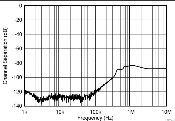
6-31. Channel Separation
