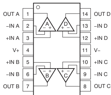
図 5-4. LMV324A-Q1 D, PW, and DYY Packages, 14-Pin SOIC, TSSOP, and SOT-23 (Top View)
